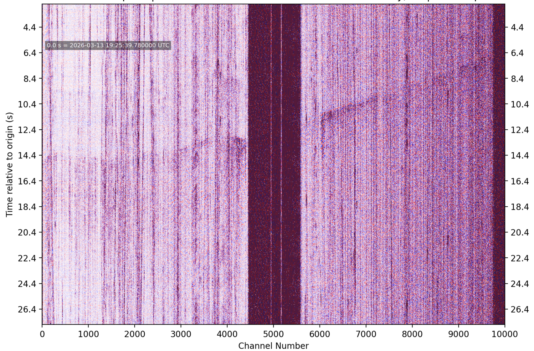
PhaseNet-DAS picks | nc75327002 M2.38 5 km WSW of Portola Valley, CA | without picks
