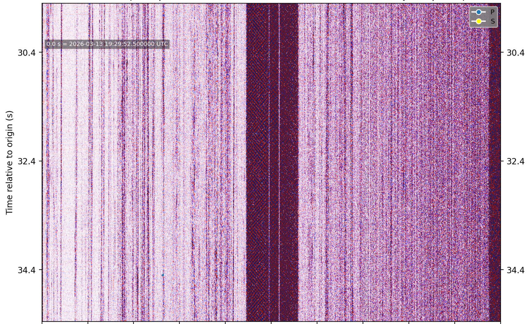
PhaseNet-DAS picks | nc75327007 M1.21 5 km WSW of Portola Valley, CA | without picks
