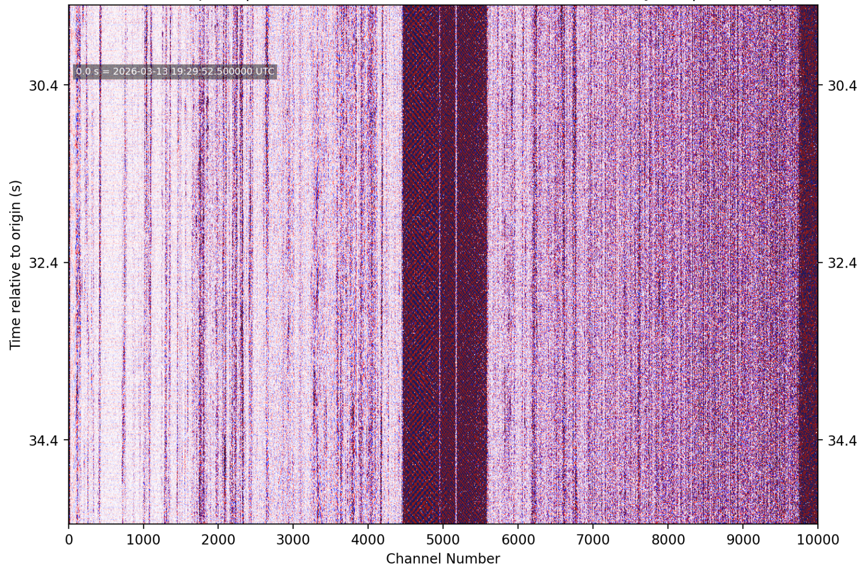
PhaseNet-DAS picks | nc75327007 M1.21 5 km WSW of Portola Valley, CA | without picks
