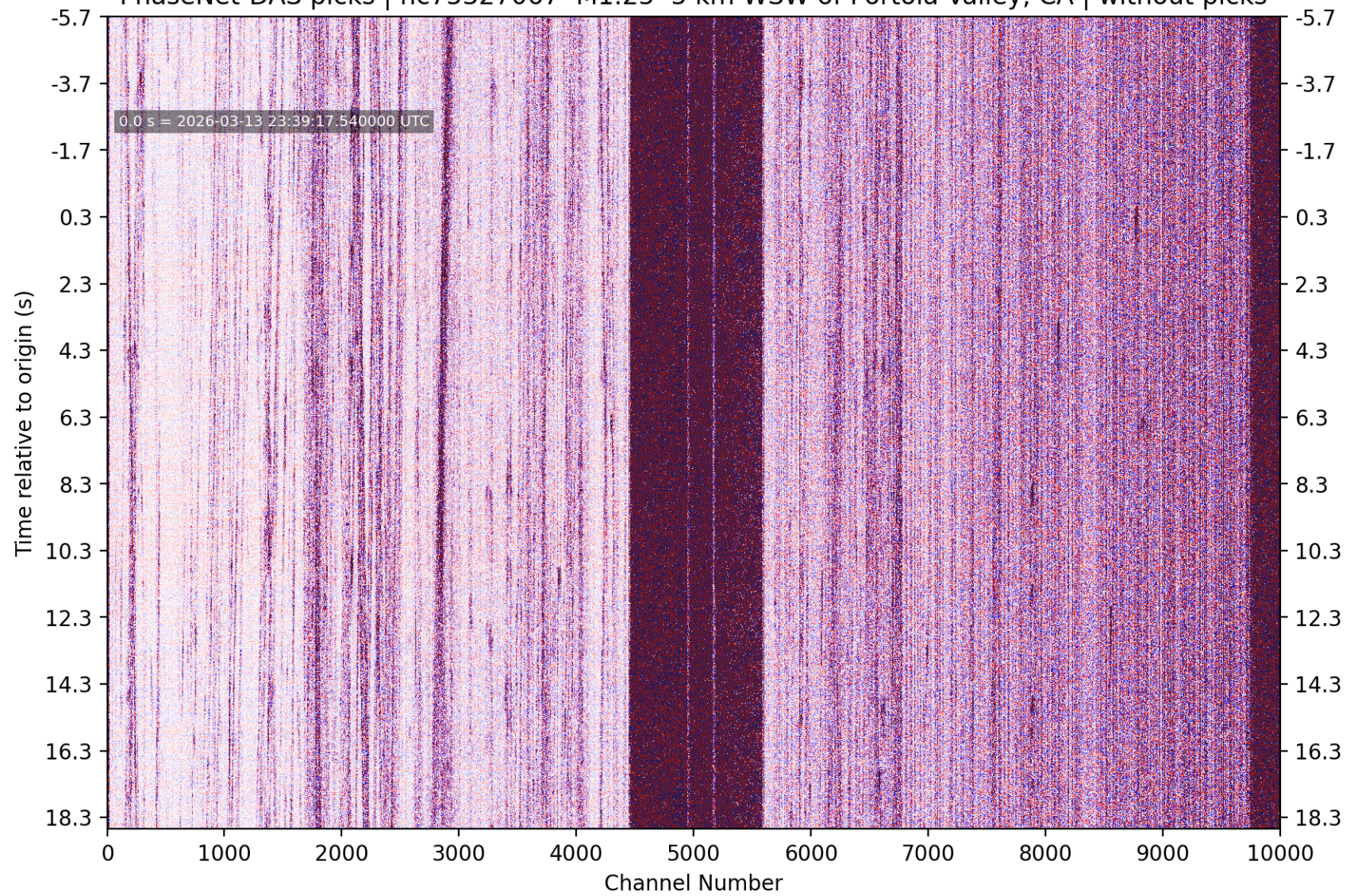
PhaseNet-DAS picks | nc75327067 M1.25 5 km WSW of Portola Valley, CA | without picks
