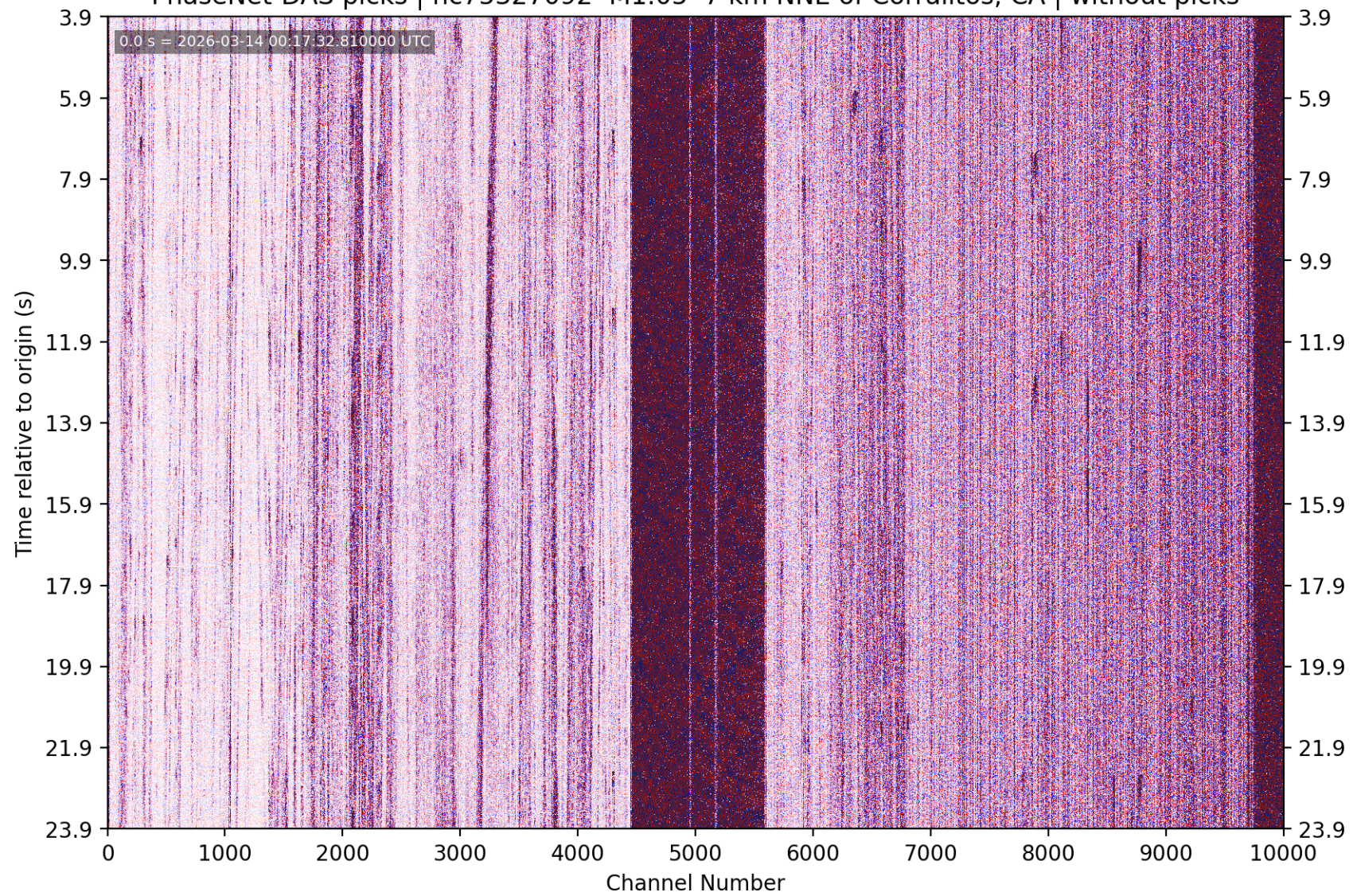
PhaseNet-DAS picks | nc75327092 M1.05 7 km NNE of Corralitos, CA | without picks
