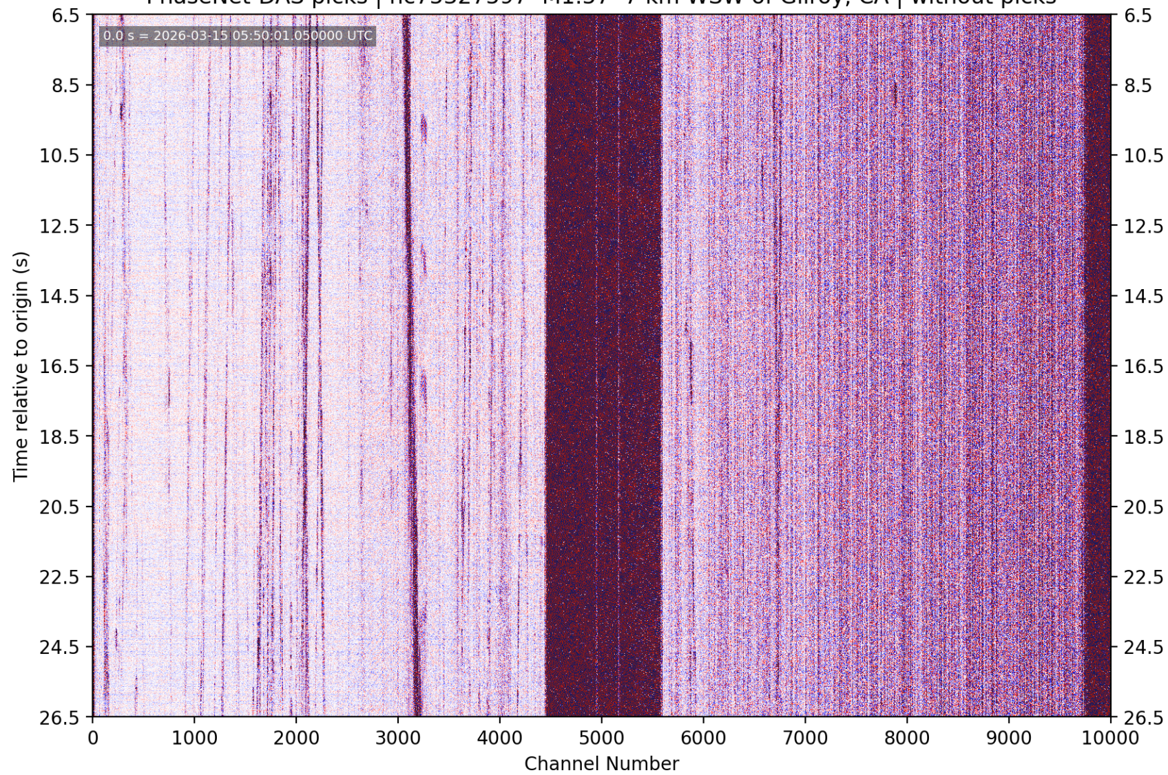
PhaseNet-DAS picks | nc75327597 M1.57 7 km WSW of Gilroy, CA | without picks
