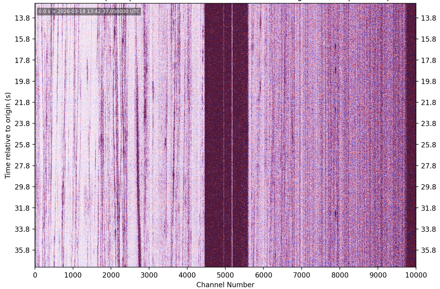
PhaseNet-DAS picks | nc75329592 M1.73 15 km NNE of Morgan Hill, CA | without picks
