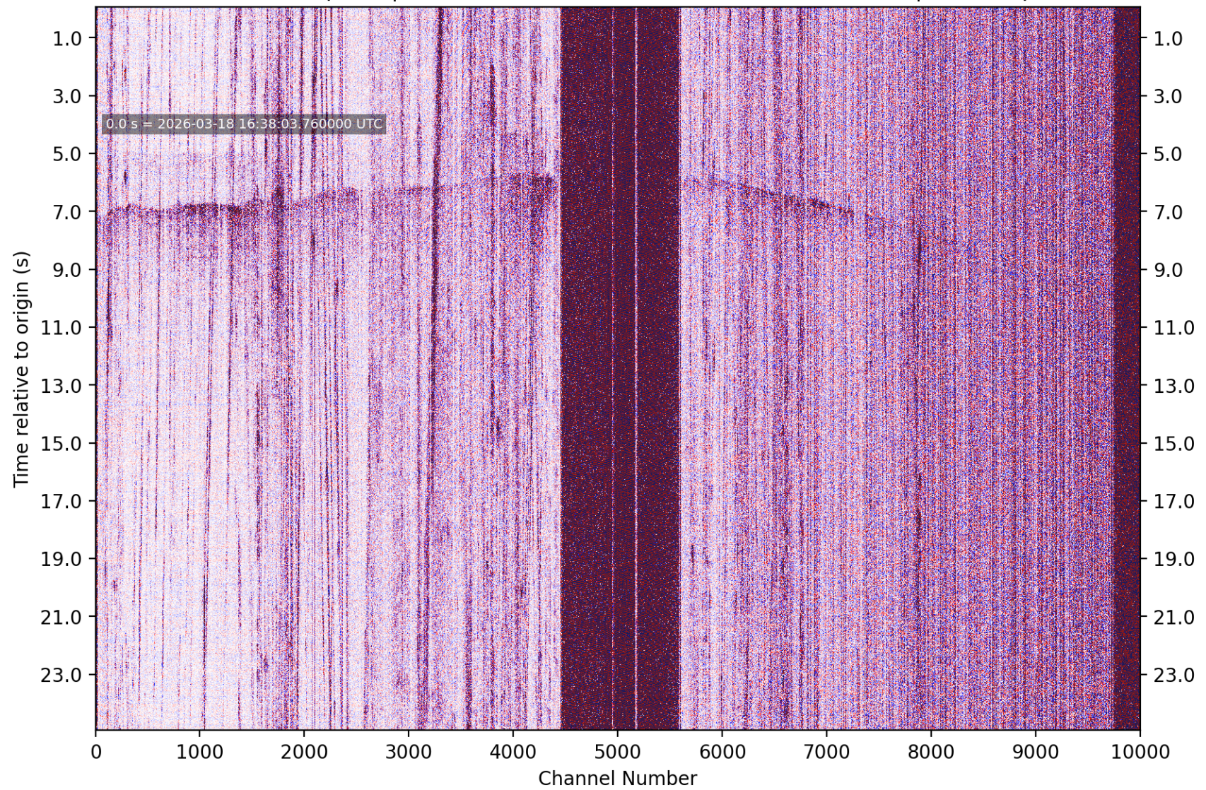
PhaseNet-DAS picks | nc75329647 M1.87 3 km SE of Pacifica, CA | without picks
