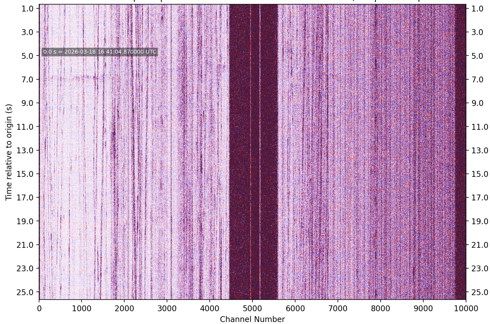
PhaseNet-DAS picks | nc75329652 M0.93 3 km SE of Pacifica, CA | without picks
