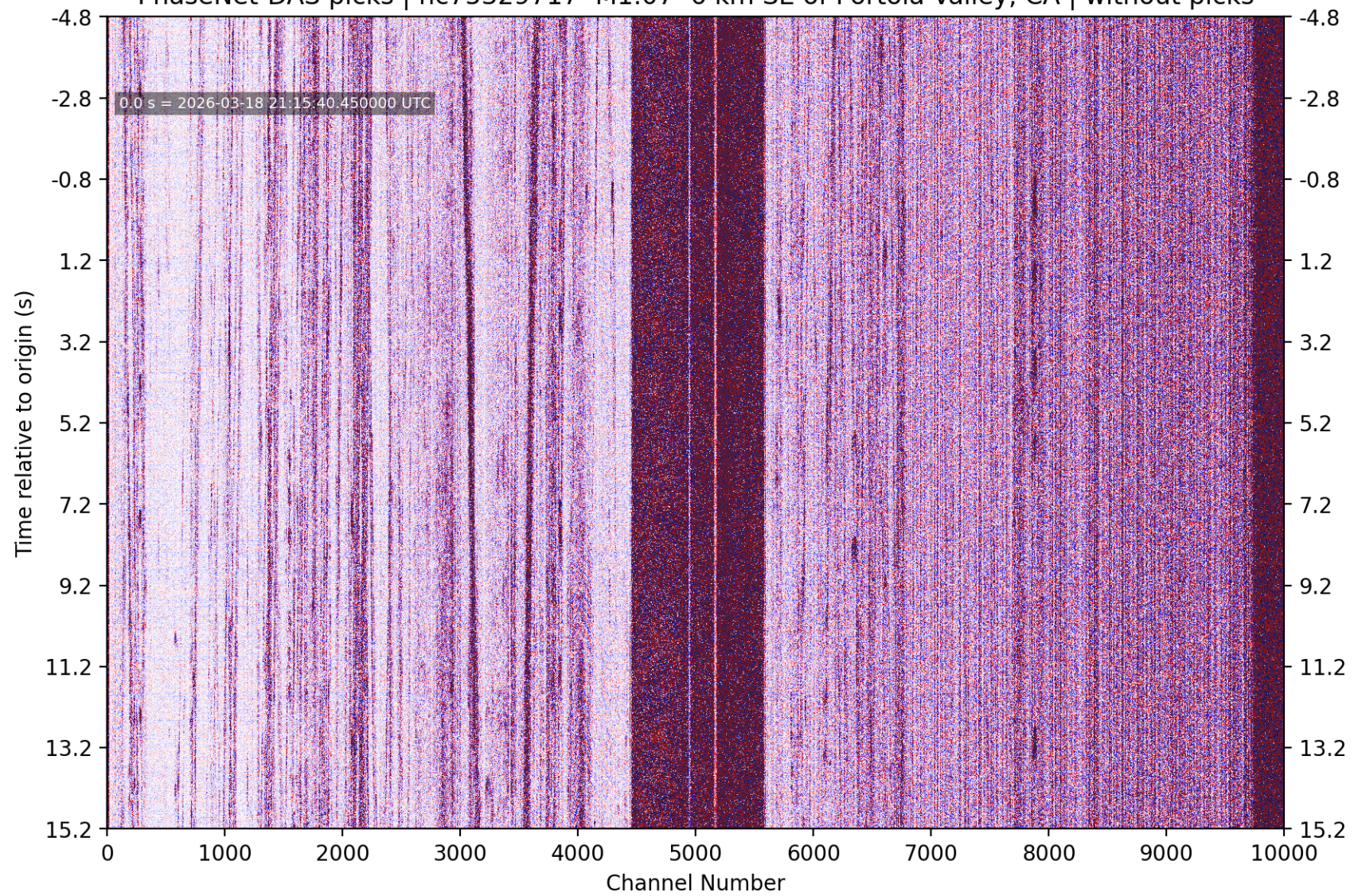
PhaseNet-DAS picks | nc75329717 M1.07 6 km SE of Portola Valley, CA | without picks
