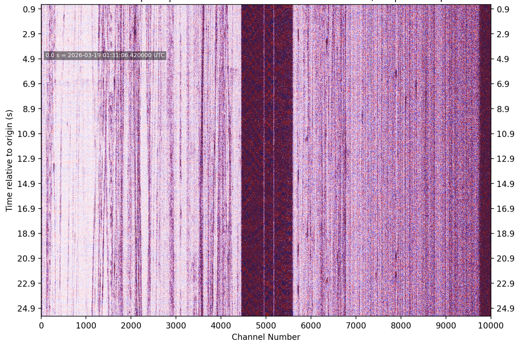
PhaseNet-DAS picks | nc75329807 M0.76 4 km SE of Pacifica, CA | without picks
