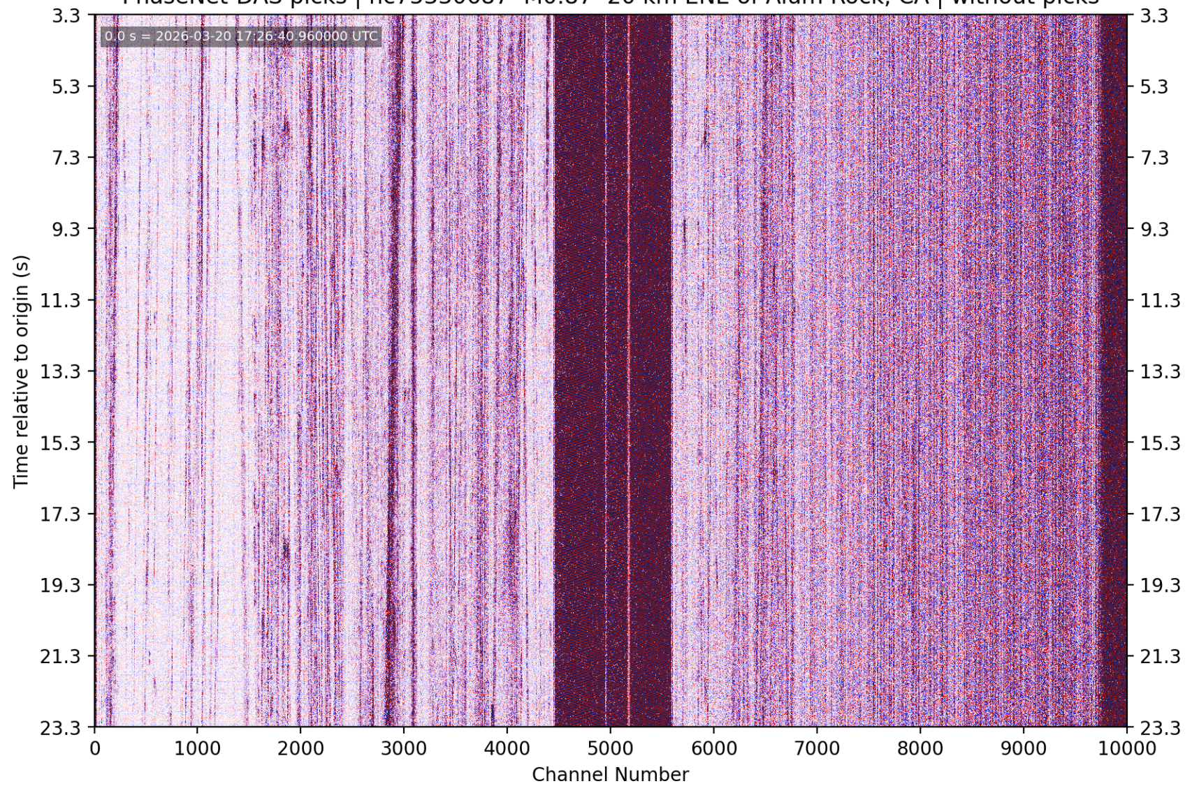
PhaseNet-DAS picks | nc75330687 M0.87 20 km ENE of Alum Rock, CA | without picks
