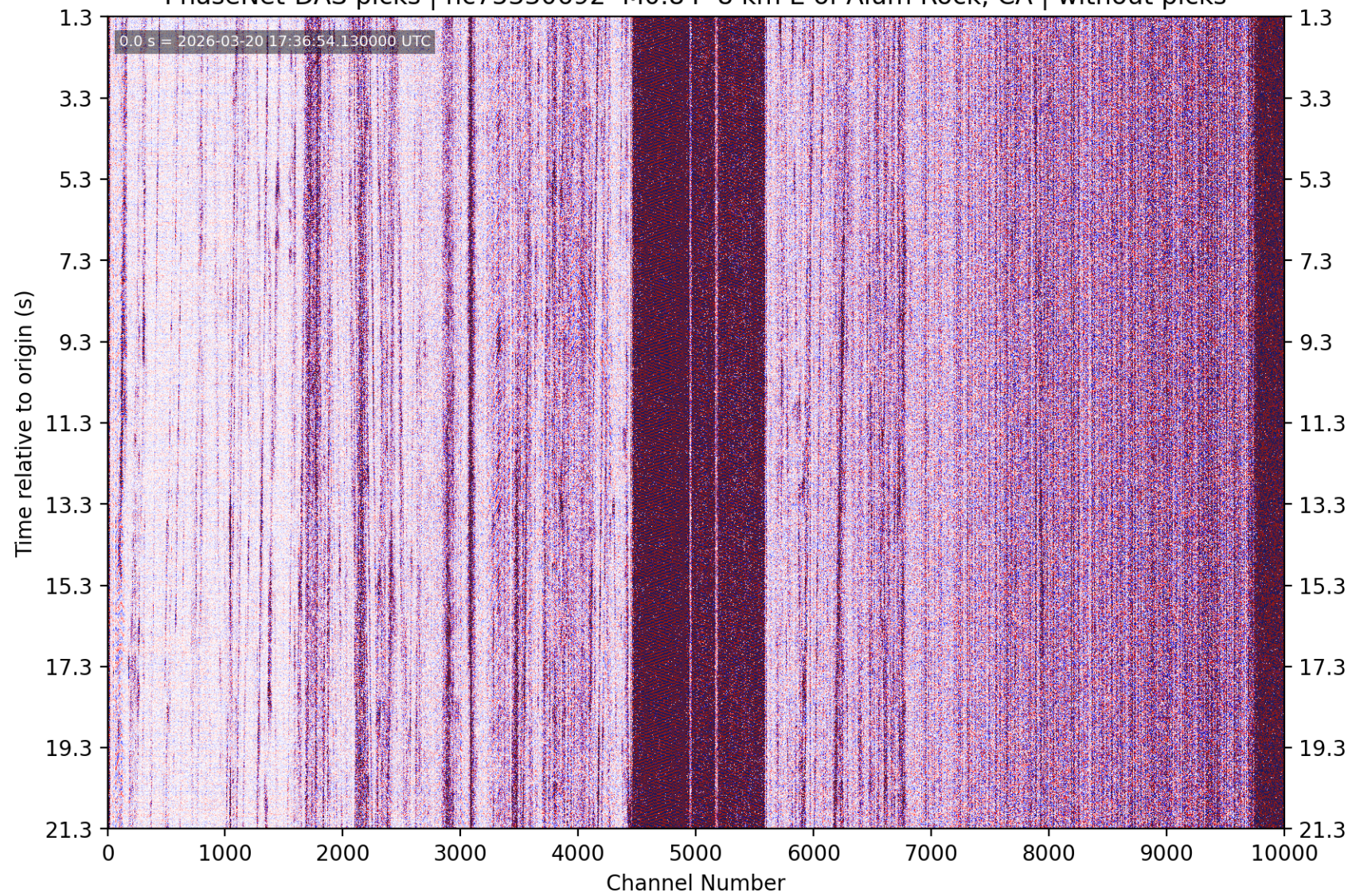
PhaseNet-DAS picks | nc75330692 M0.84 8 km E of Alum Rock, CA | without picks
