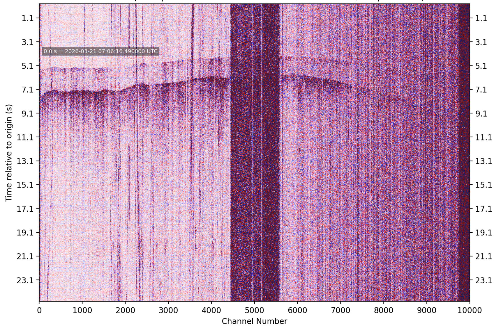
PhaseNet-DAS picks | nc75330912 M1.76 5 km SE of Pacifica, CA | without picks
