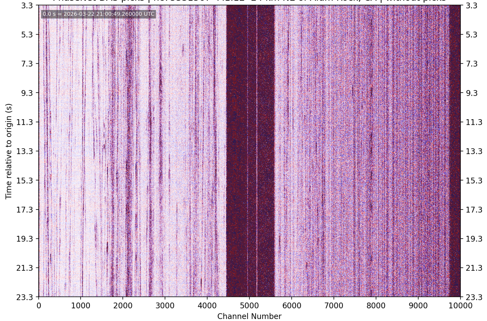
PhaseNet-DAS picks | nc75331567 M1.12 24 km NE of Alum Rock, CA | without picks
