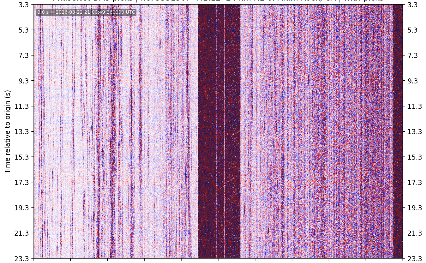
PhaseNet-DAS picks | nc75331567 M1.12 24 km NE of Alum Rock, CA | without picks
