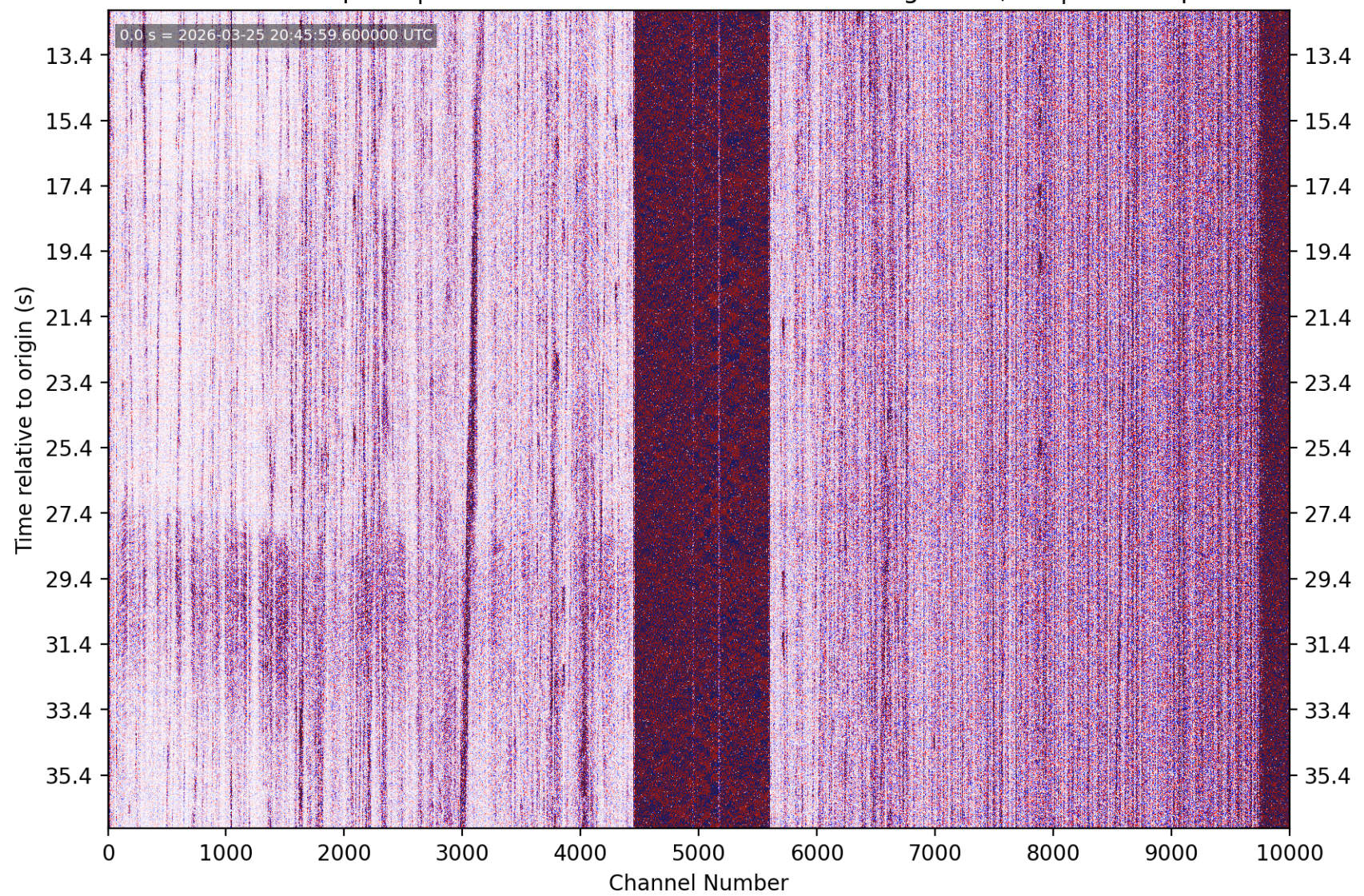
PhaseNet-DAS picks | nc75332922 M2.46 15 km N of Morgan Hill, CA | without picks
