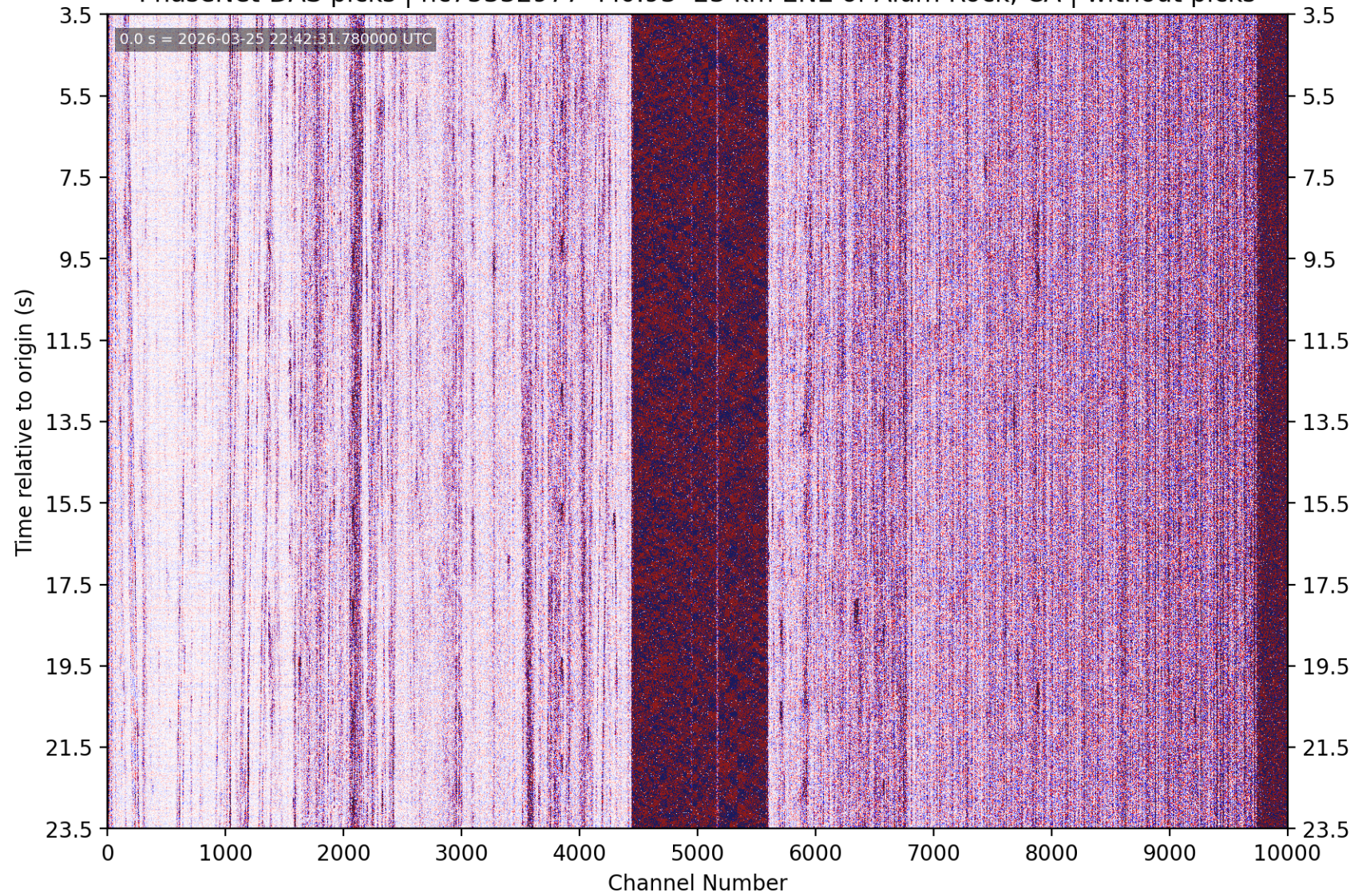
PhaseNet-DAS picks | nc75332977 M0.93 23 km ENE of Alum Rock, CA | without picks
