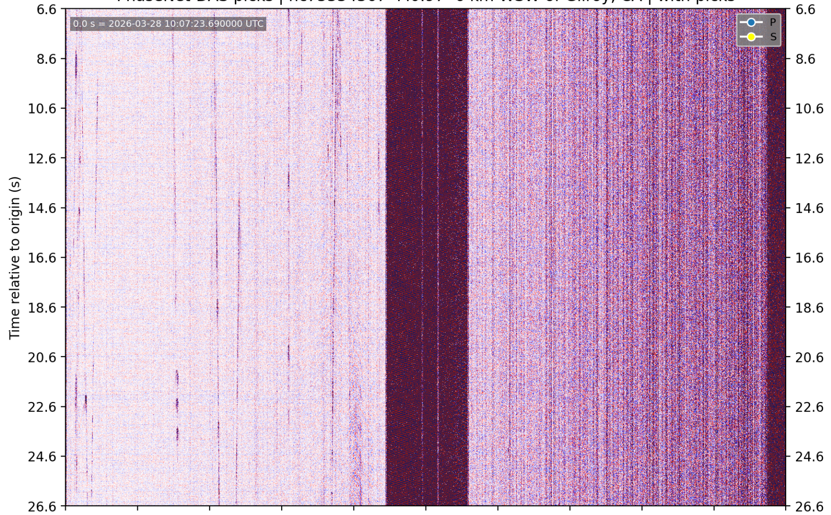
PhaseNet-DAS picks | nc75334367 M0.97 6 km WSW of Gilroy, CA | without picks
