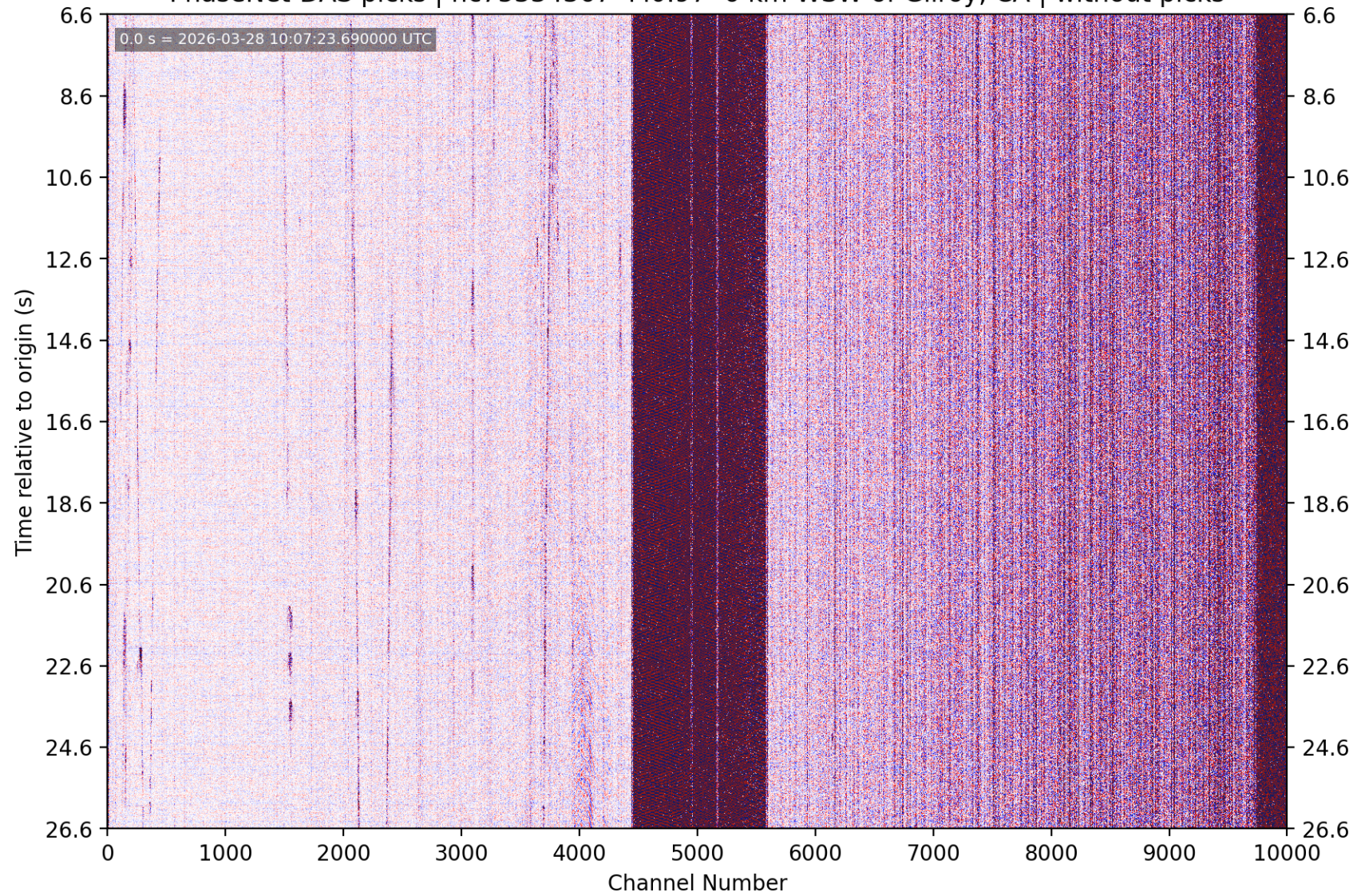
PhaseNet-DAS picks | nc75334367 M0.97 6 km WSW of Gilroy, CA | without picks
