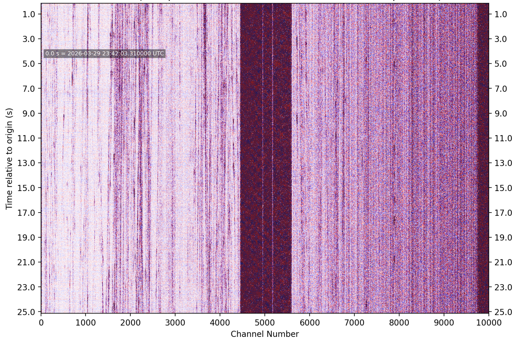
PhaseNet-DAS picks | nc75335237 M0.54 3 km SE of Pacifica, CA | without picks
