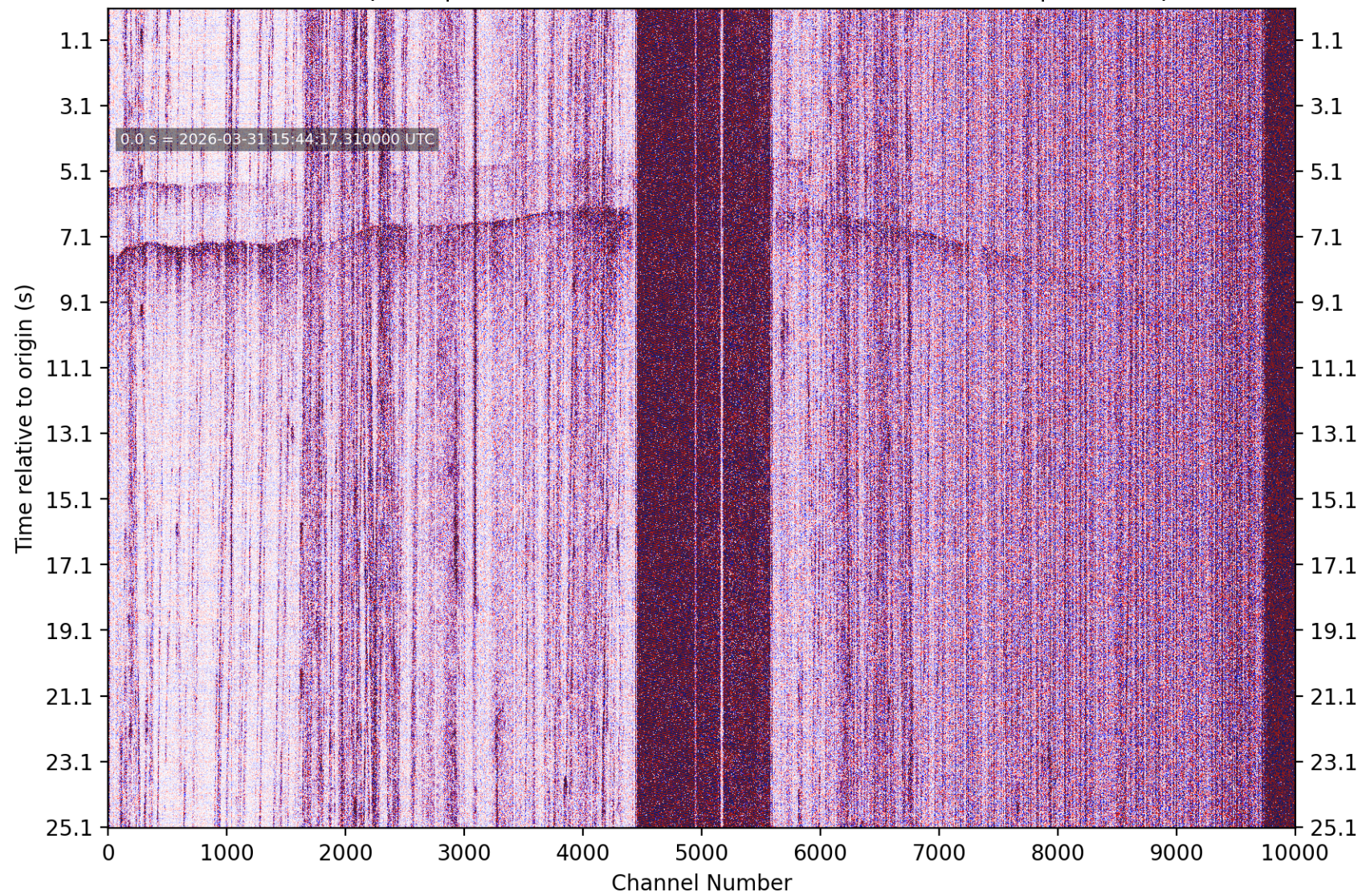
PhaseNet-DAS picks | nc75336292 M1.59 4 km SE of Pacifica, CA | without picks
