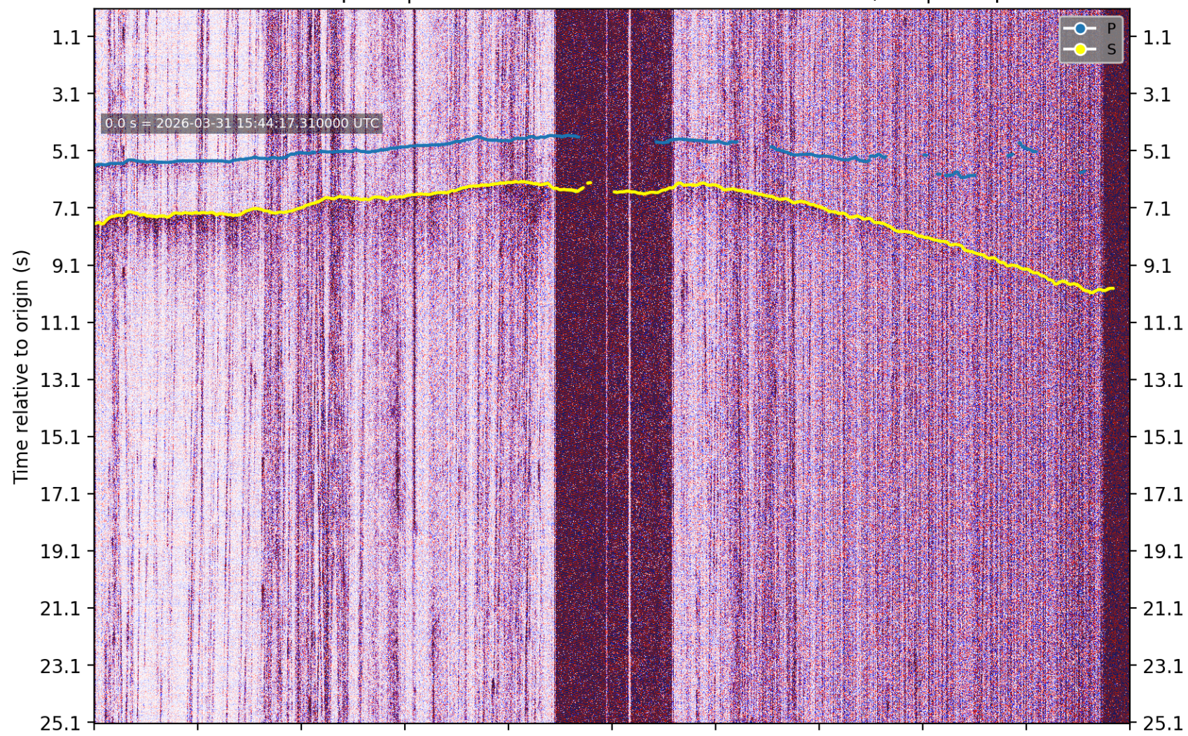
PhaseNet-DAS picks | nc75336292 M1.59 4 km SE of Pacifica, CA | without picks
