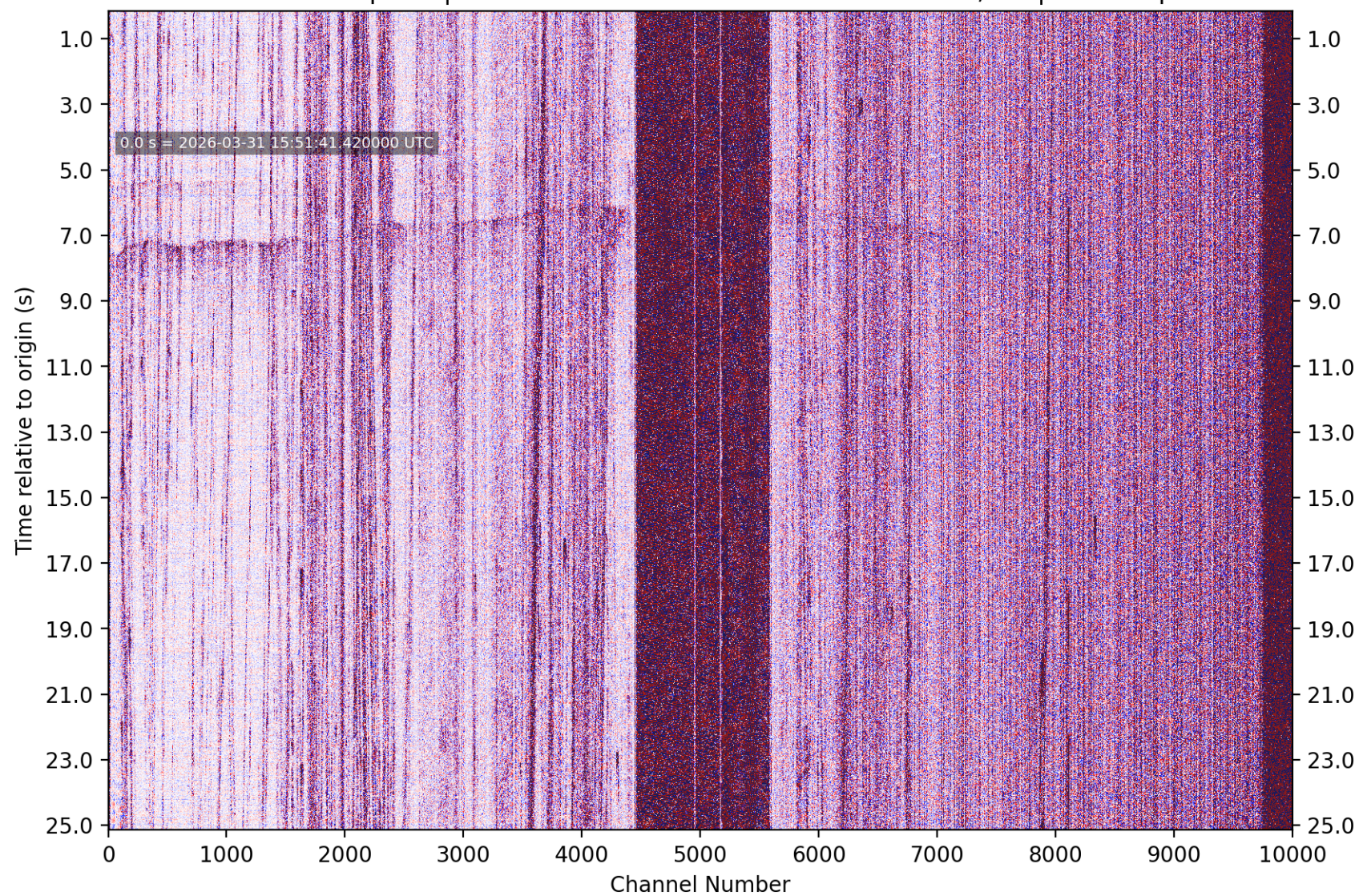
PhaseNet-DAS picks | nc75336302 M1.35 4 km SE of Pacifica, CA | without picks
