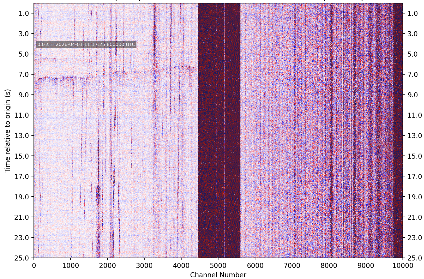
PhaseNet-DAS picks | nc75336932 M1.17 4 km SE of Pacifica, CA | without picks
