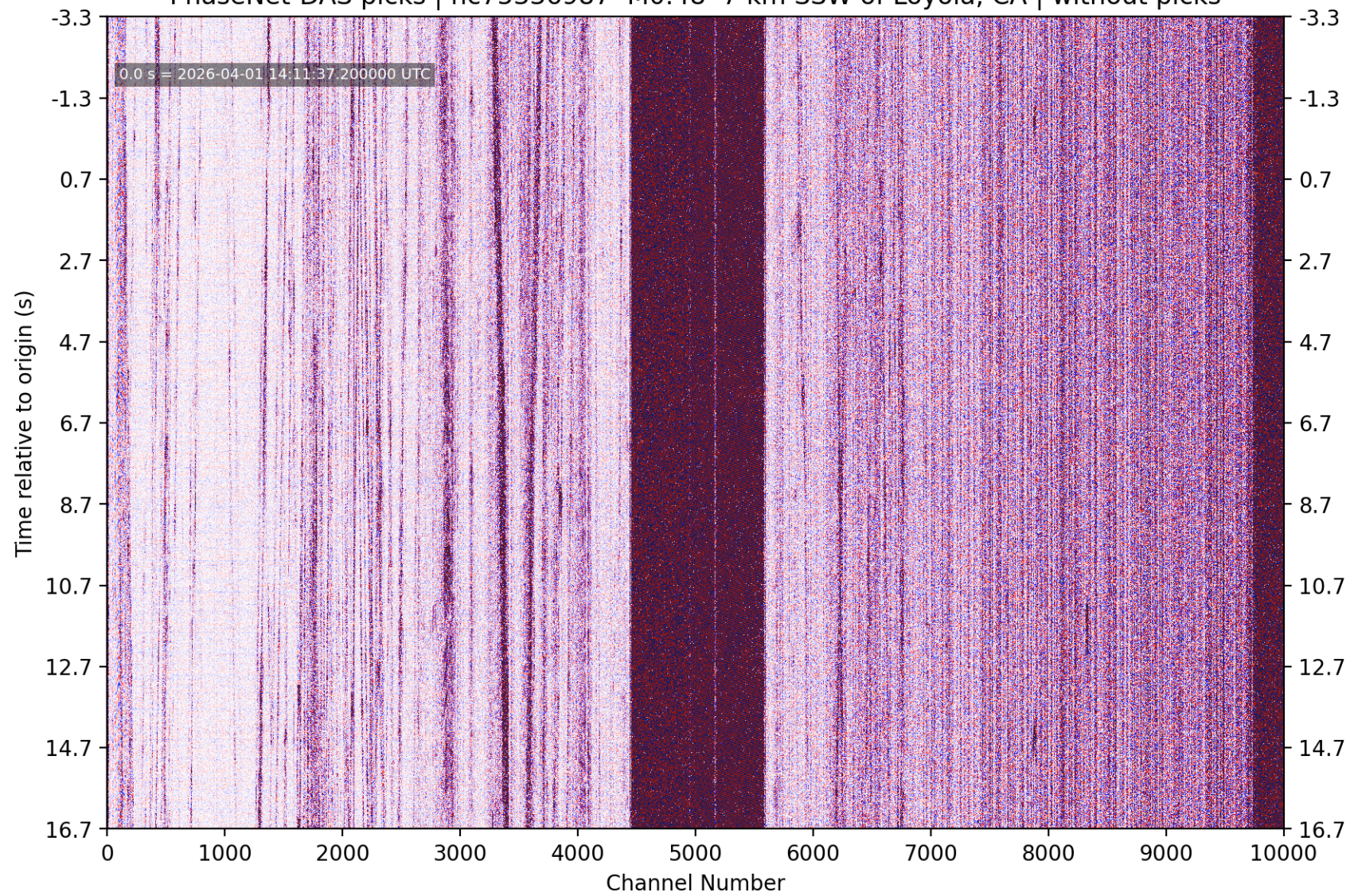
PhaseNet-DAS picks | nc75336987 M0.48 7 km SSW of Loyola, CA | without picks
