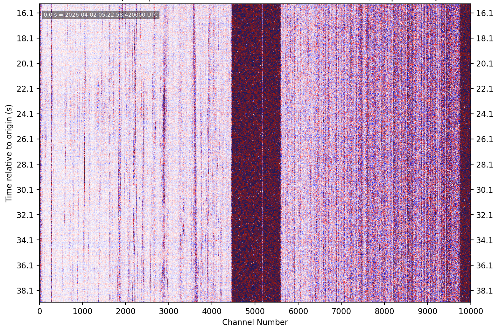
PhaseNet-DAS picks | nc75337397 M1.92 9 km N of Boulder Creek, CA | without picks
