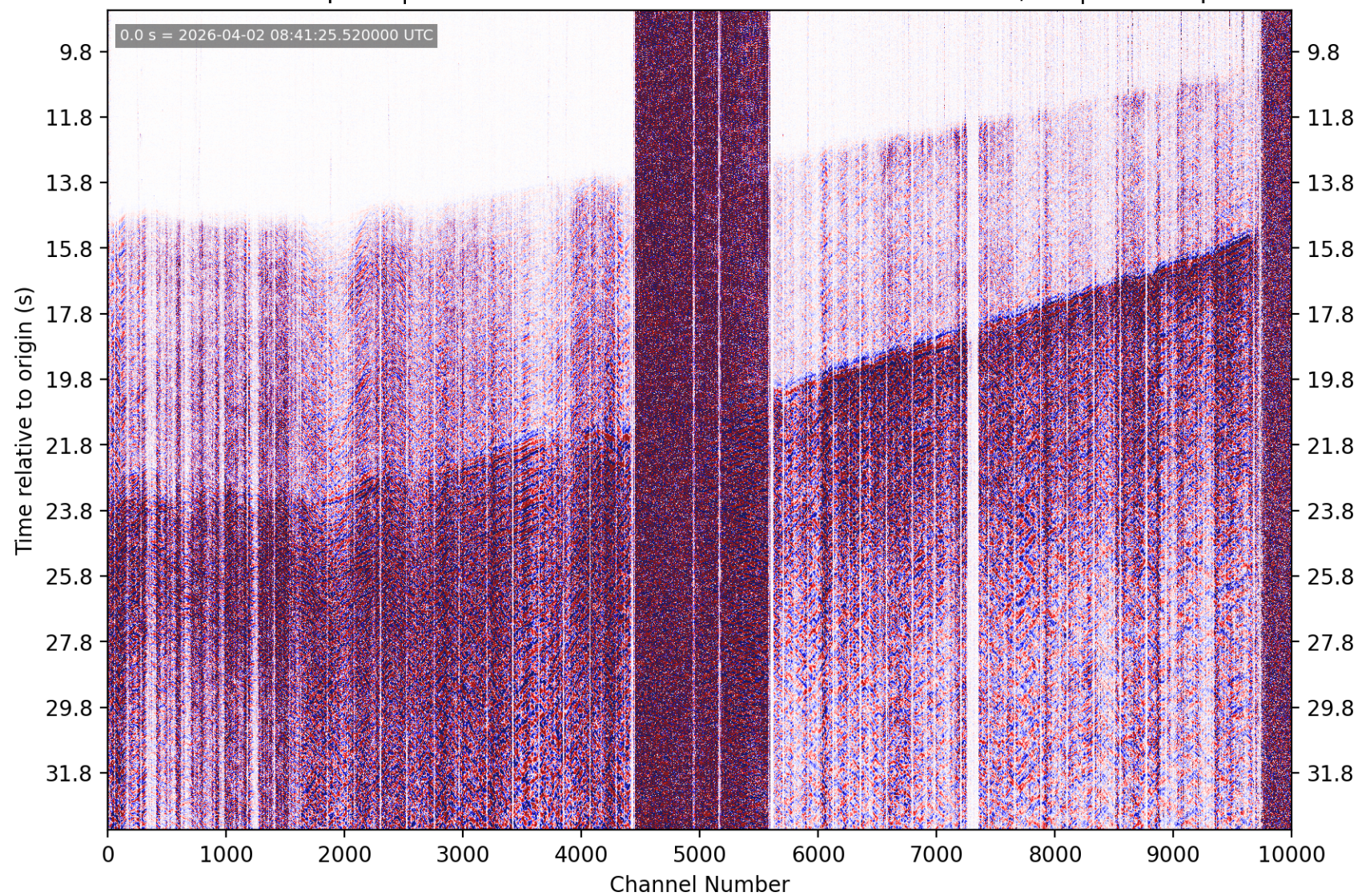
PhaseNet-DAS picks | nc75337442 M4.59 1 km SE of Boulder Creek, CA | without picks
