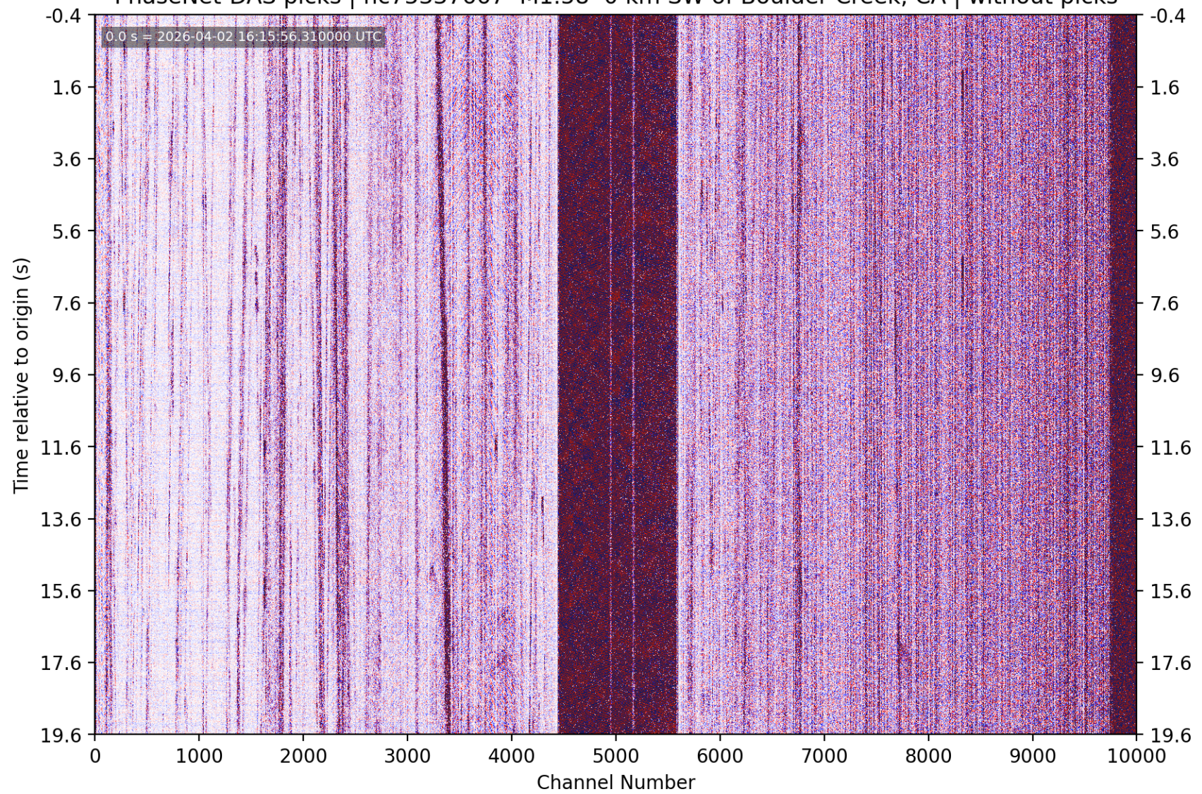
PhaseNet-DAS picks | nc75337667 M1.58 0 km SW of Boulder Creek, CA | without picks
