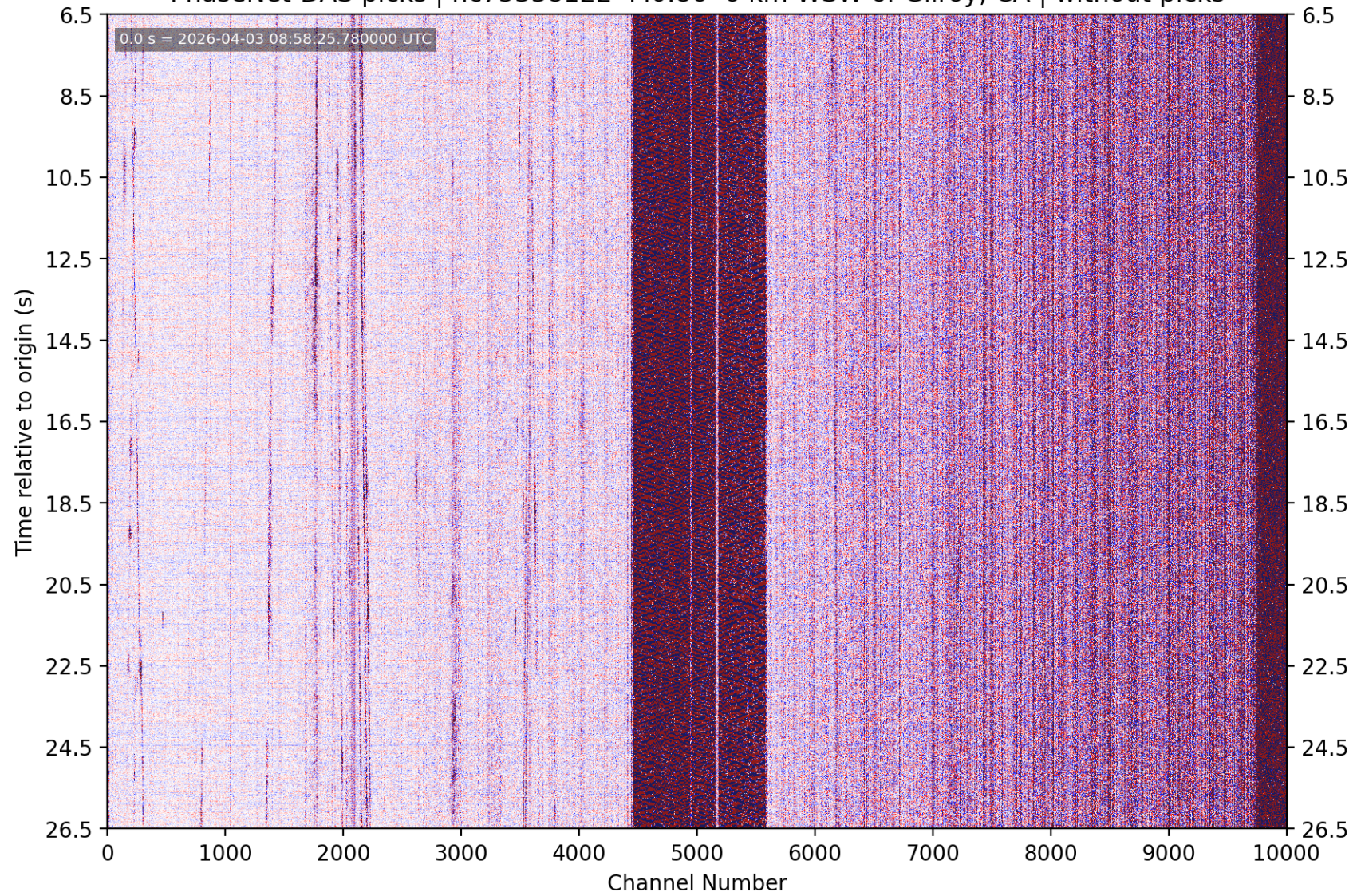
PhaseNet-DAS picks | nc75338122 M0.86 6 km WSW of Gilroy, CA | without picks
