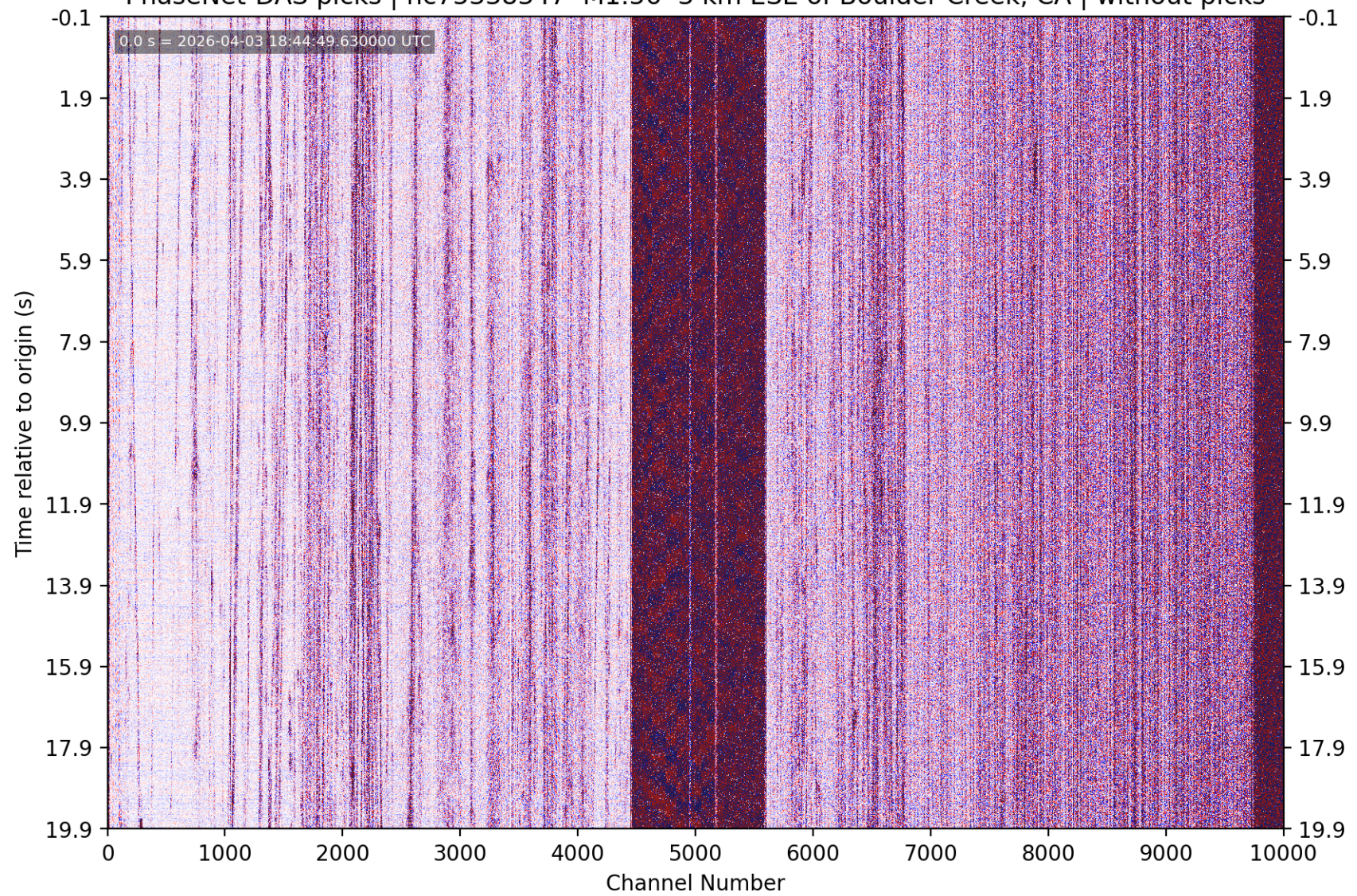
PhaseNet-DAS picks | nc75338347 M1.56 3 km ESE of Boulder Creek, CA | without picks
