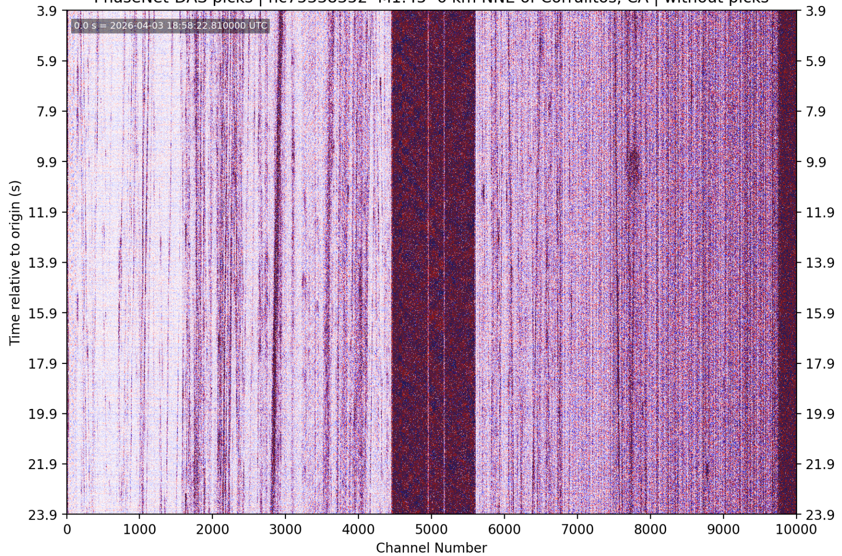
PhaseNet-DAS picks | nc75338352 M1.45 6 km NNE of Corralitos, CA | without picks
