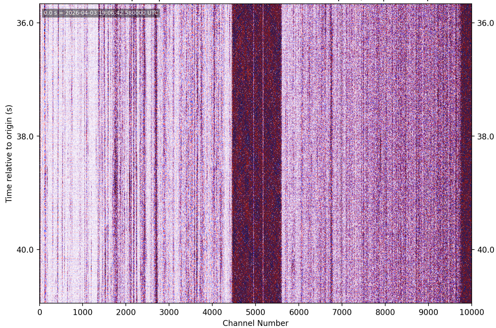
PhaseNet-DAS picks | nc75338362 M1.59 9 km ENE of Milpitas, CA | without picks
