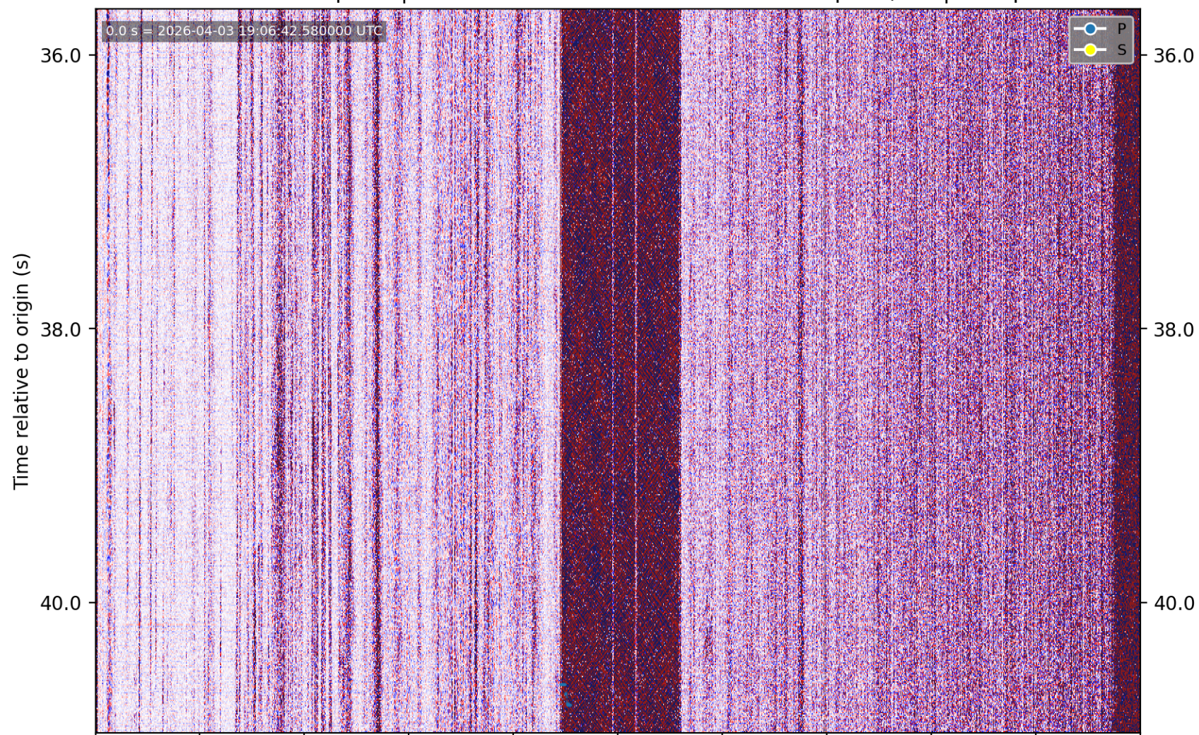
PhaseNet-DAS picks | nc75338362 M1.59 9 km ENE of Milpitas, CA | without picks
