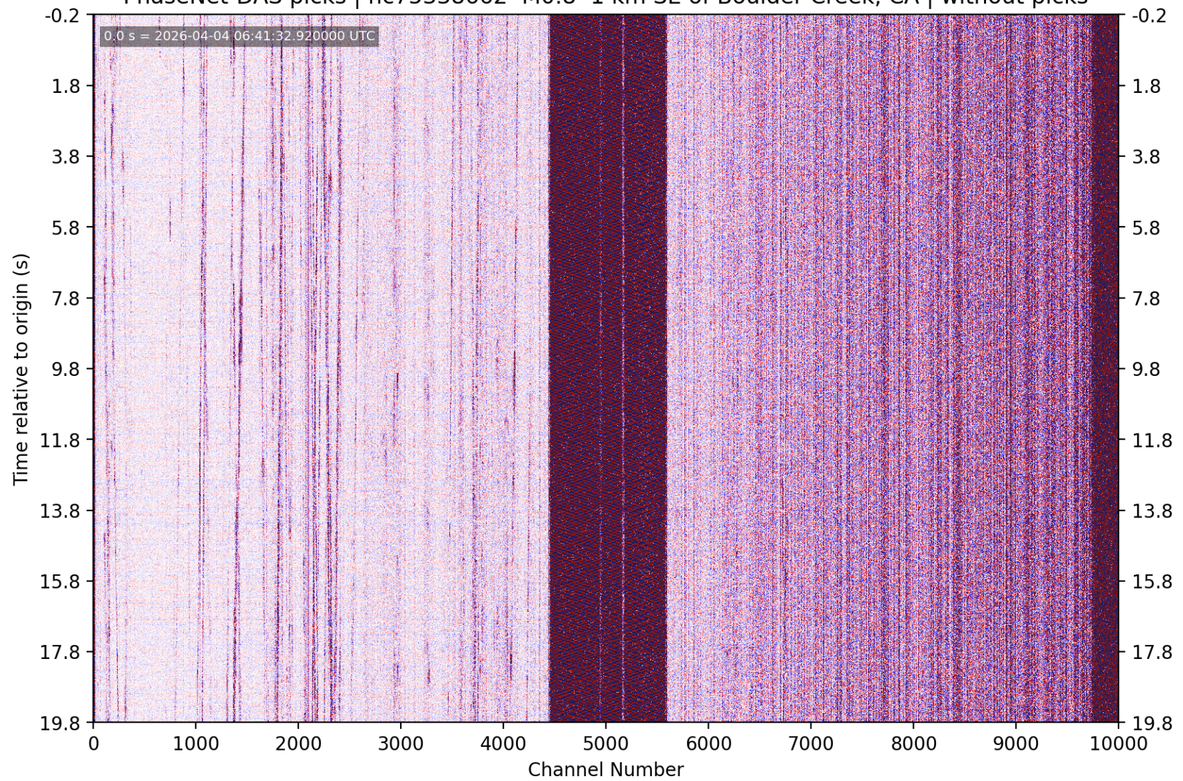
PhaseNet-DAS picks | nc75338662 M0.8 1 km SE of Boulder Creek, CA | without picks
