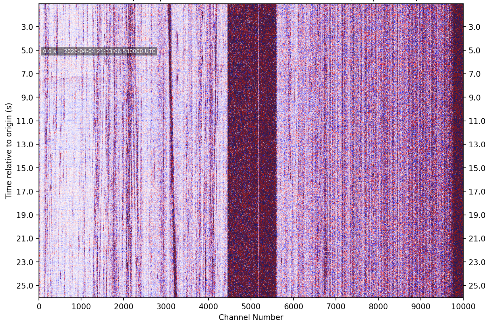
PhaseNet-DAS picks | nc75339017 M1.23 4 km SE of Pacifica, CA | without picks
