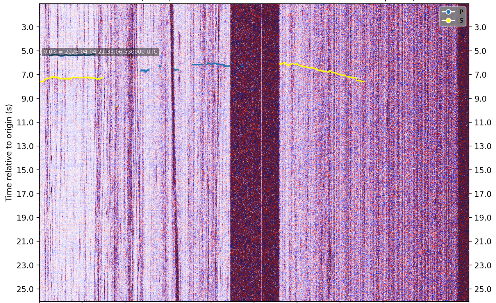
PhaseNet-DAS picks | nc75339017 M1.23 4 km SE of Pacifica, CA | without picks
