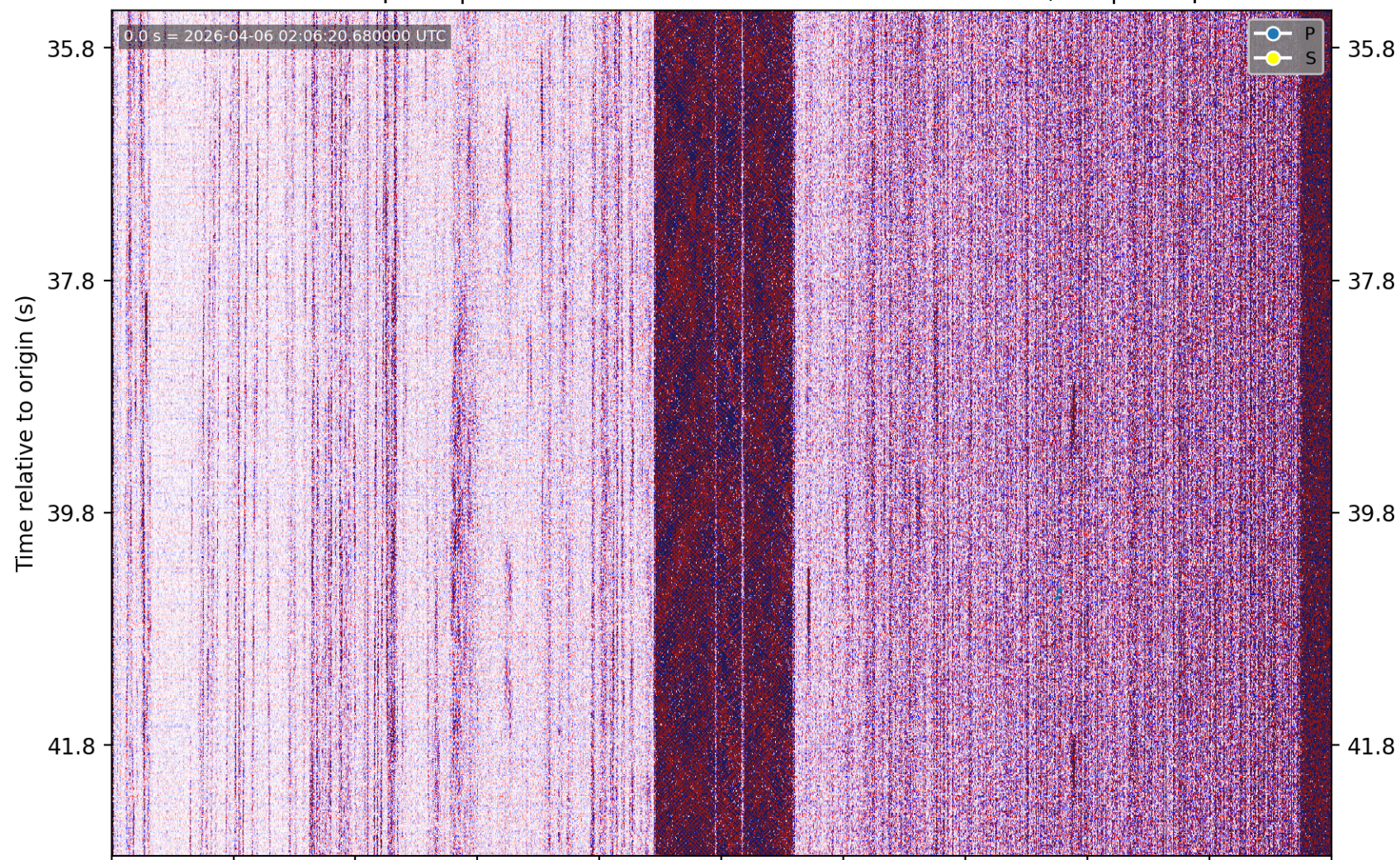
PhaseNet-DAS picks | nc75339592 M0.97 10 km E of Alum Rock, CA | without picks
