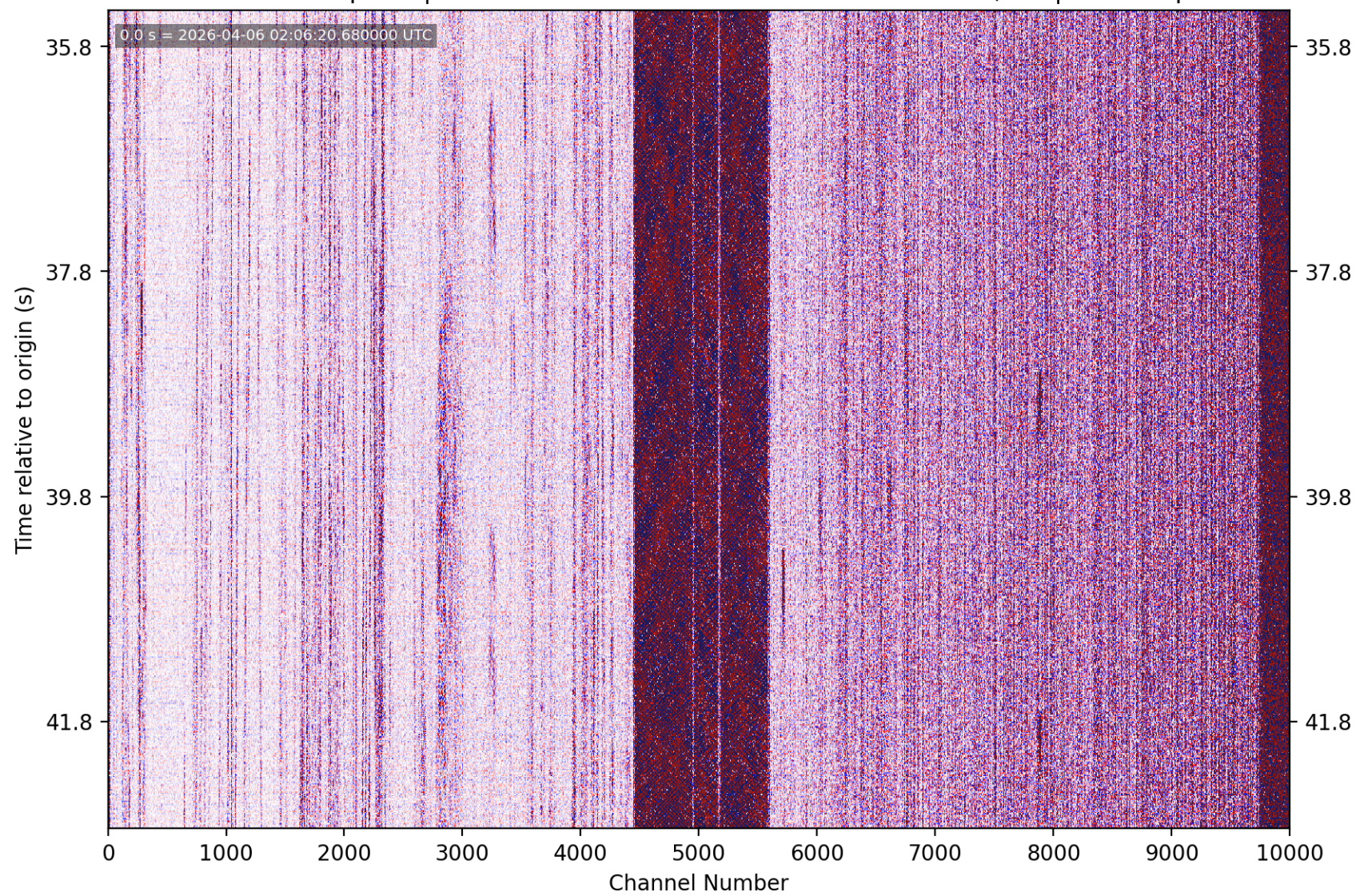
PhaseNet-DAS picks | nc75339592 M0.97 10 km E of Alum Rock, CA | without picks
