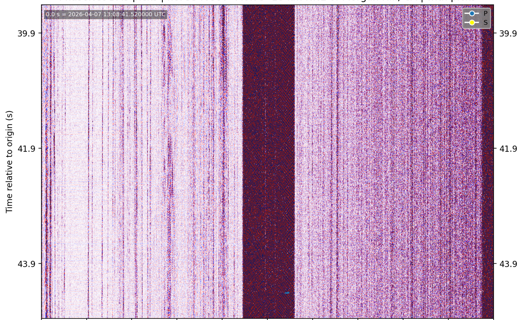
PhaseNet-DAS picks | nc75340397 M0.79 18 km NNE of Morgan Hill, CA | without picks
