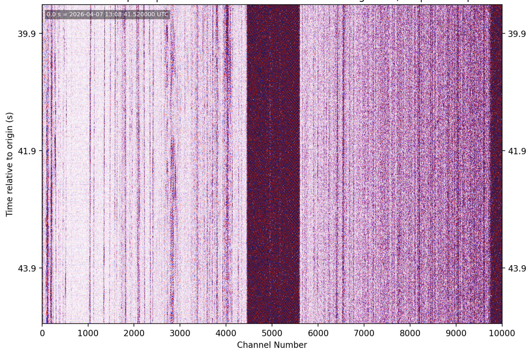
PhaseNet-DAS picks | nc75340397 M0.79 18 km NNE of Morgan Hill, CA | without picks
