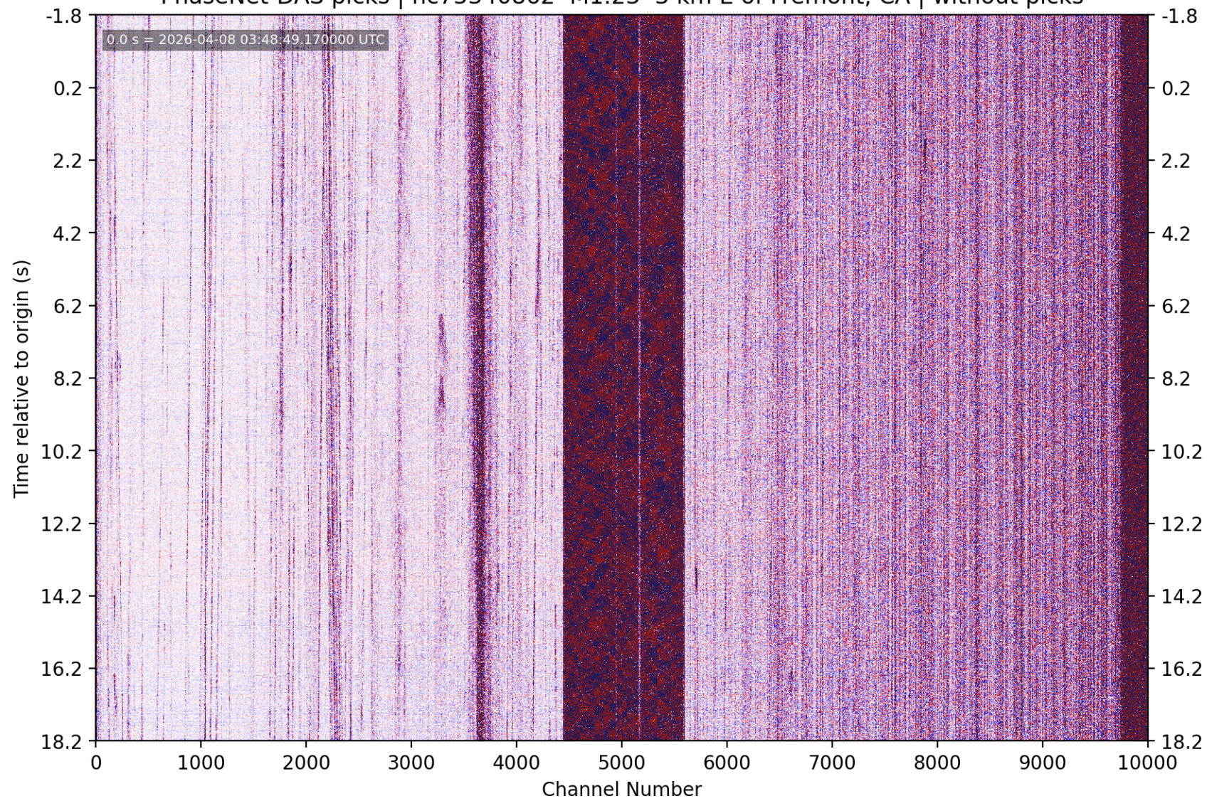
PhaseNet-DAS picks | nc75340862 M1.23 3 km E of Fremont, CA | without picks
