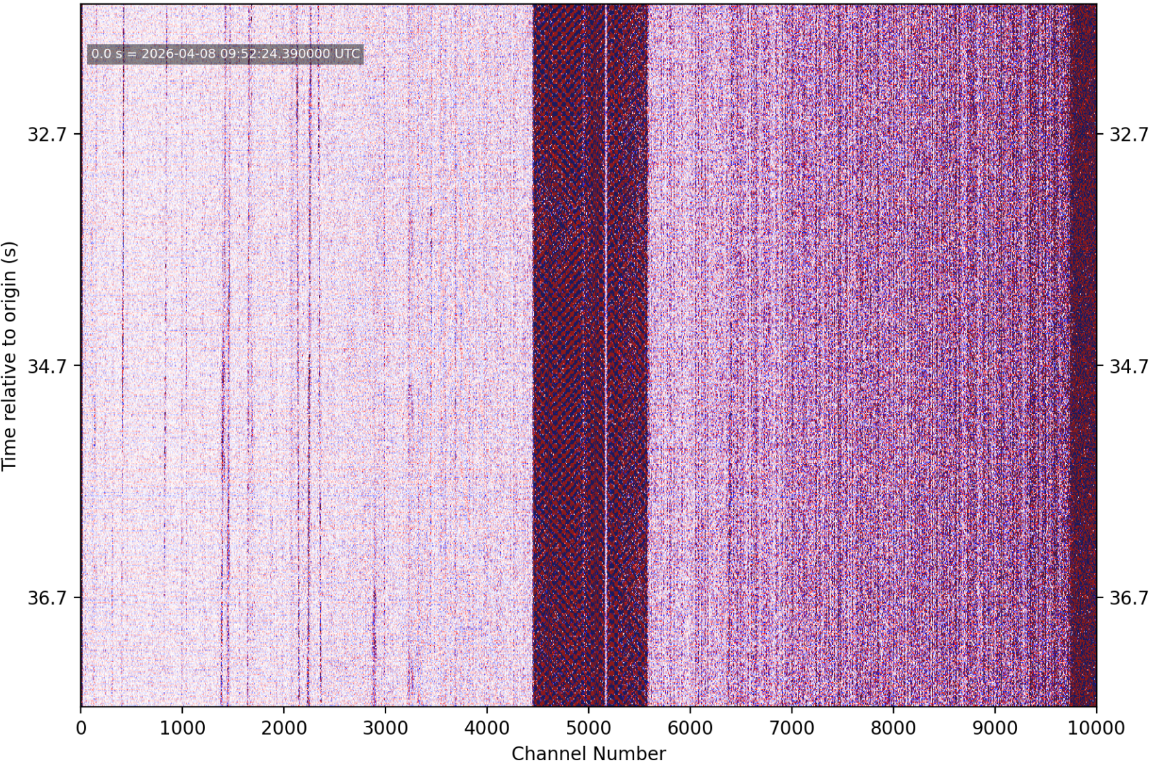
PhaseNet-DAS picks | nc75340952 M0.17 11 km SSW of Loyola, CA | without picks
