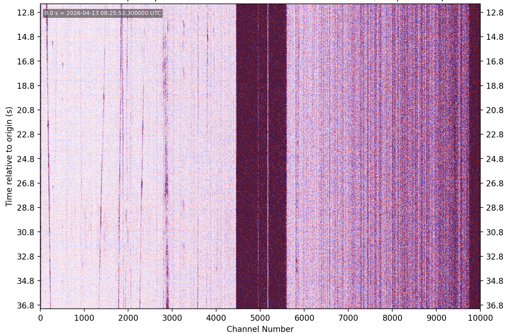
PhaseNet-DAS picks | nc75343347 M1.79 15 km E of Seven Trees, CA | without picks
