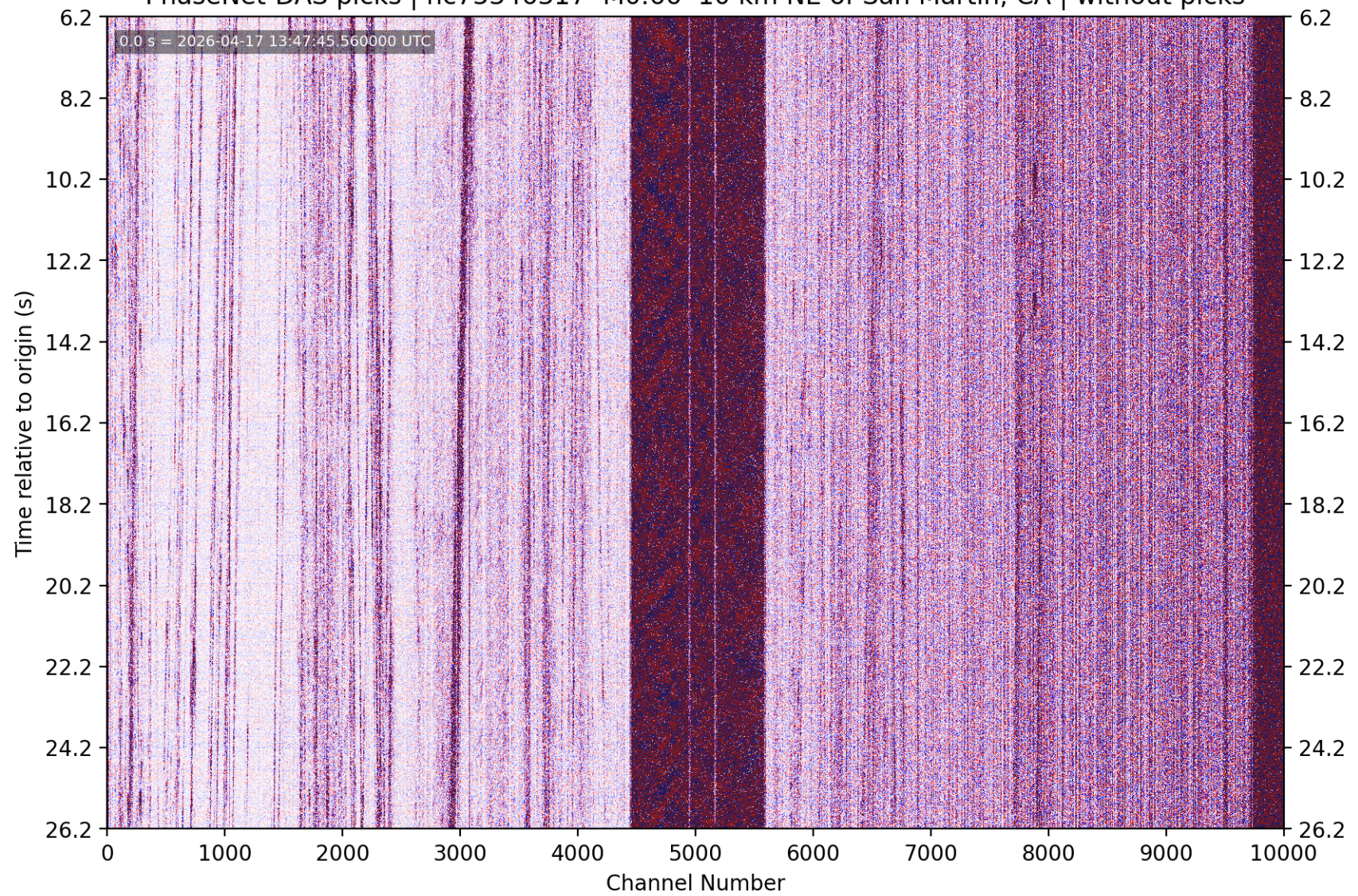
PhaseNet-DAS picks | nc75346317 M0.66 10 km NE of San Martin, CA | without picks
