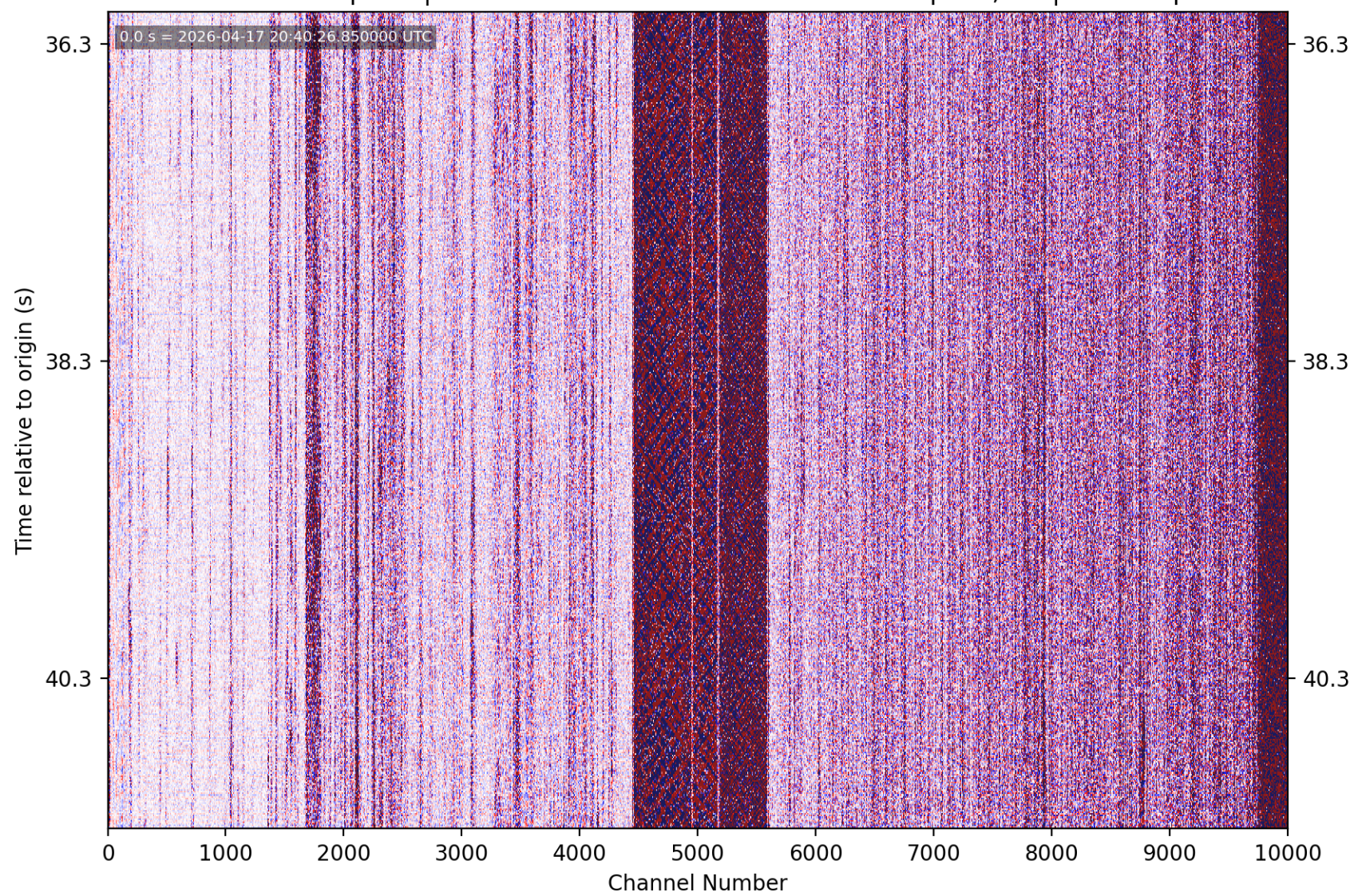
PhaseNet-DAS picks | nc75346592 M0.91 10 km ENE of Milpitas, CA | without picks
