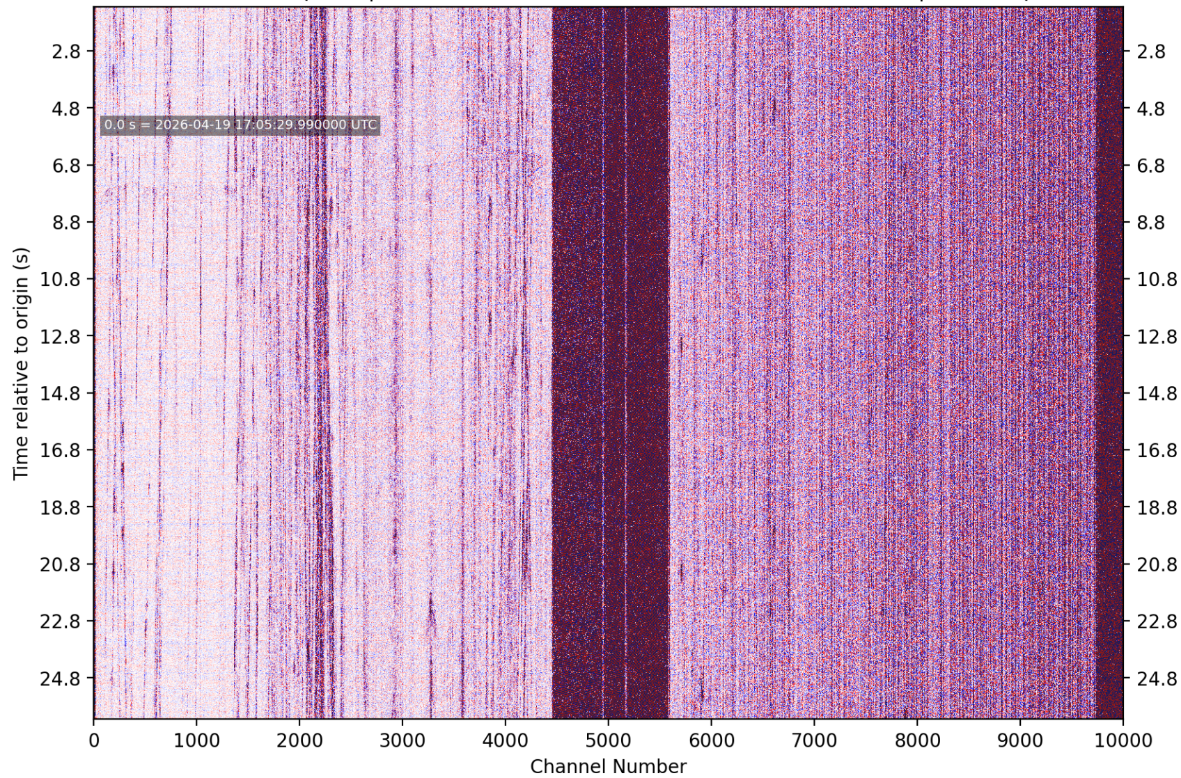
PhaseNet-DAS picks | nc75347922 M0.89 5 km WSW of Millbrae, CA | without picks
