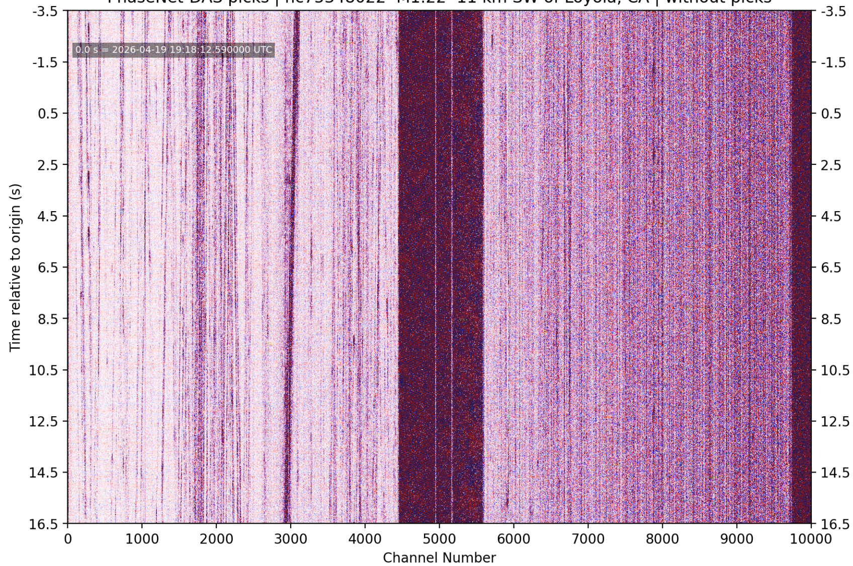
PhaseNet-DAS picks | nc75348022 M1.22 11 km SW of Loyola, CA | without picks
