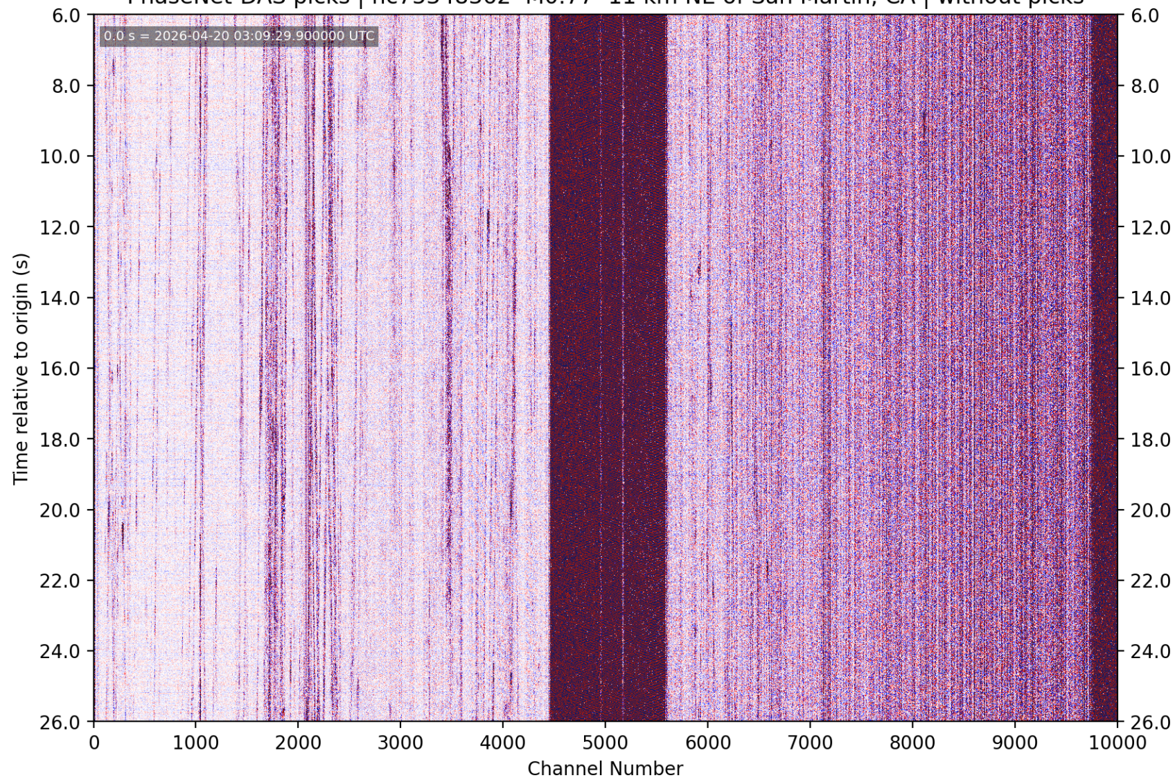
PhaseNet-DAS picks | nc75348362 M0.77 11 km NE of San Martin, CA | without picks
