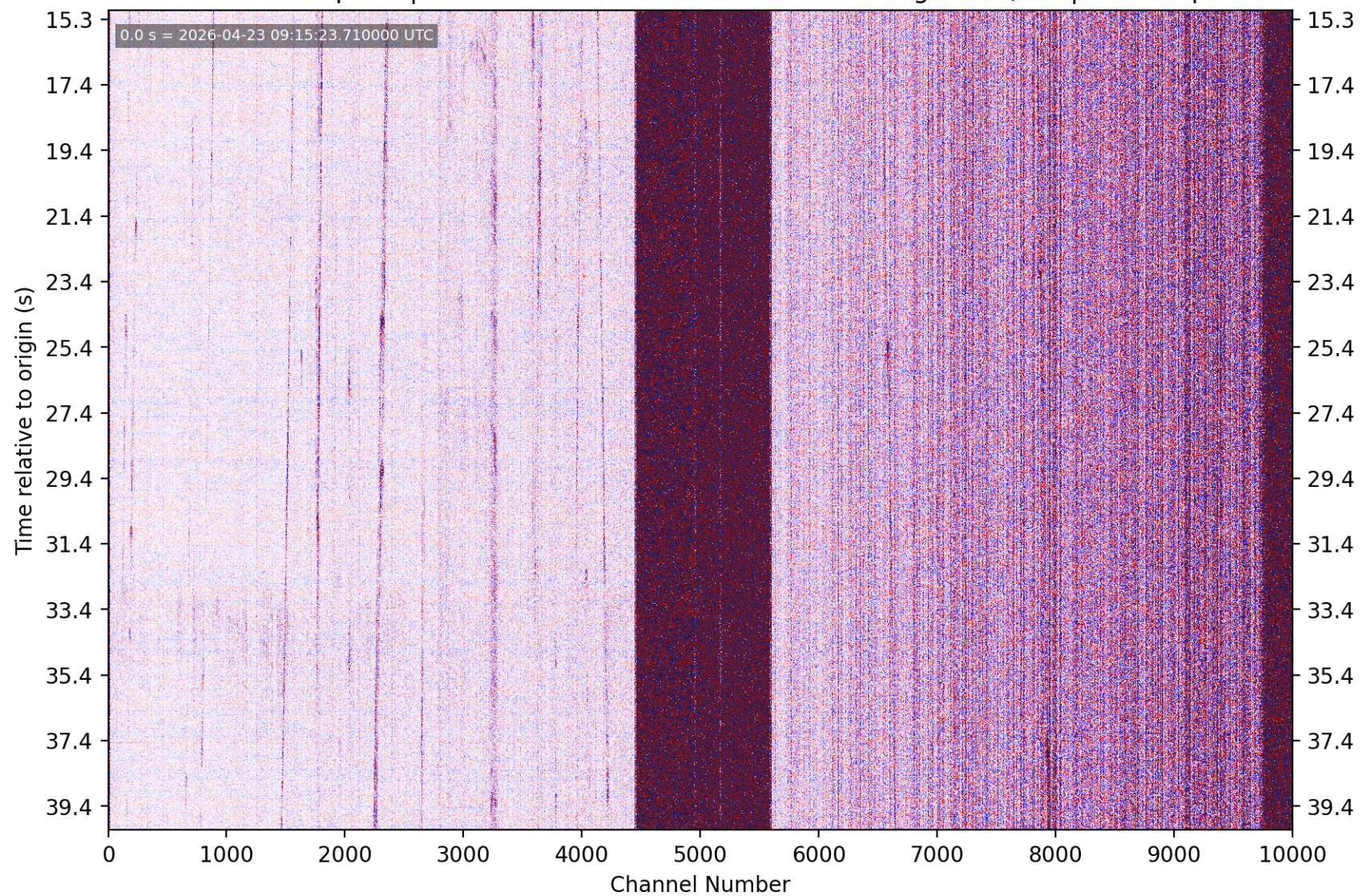
PhaseNet-DAS picks | nc75350007 M1.71 9 km ENE of Morgan Hill, CA | without picks
