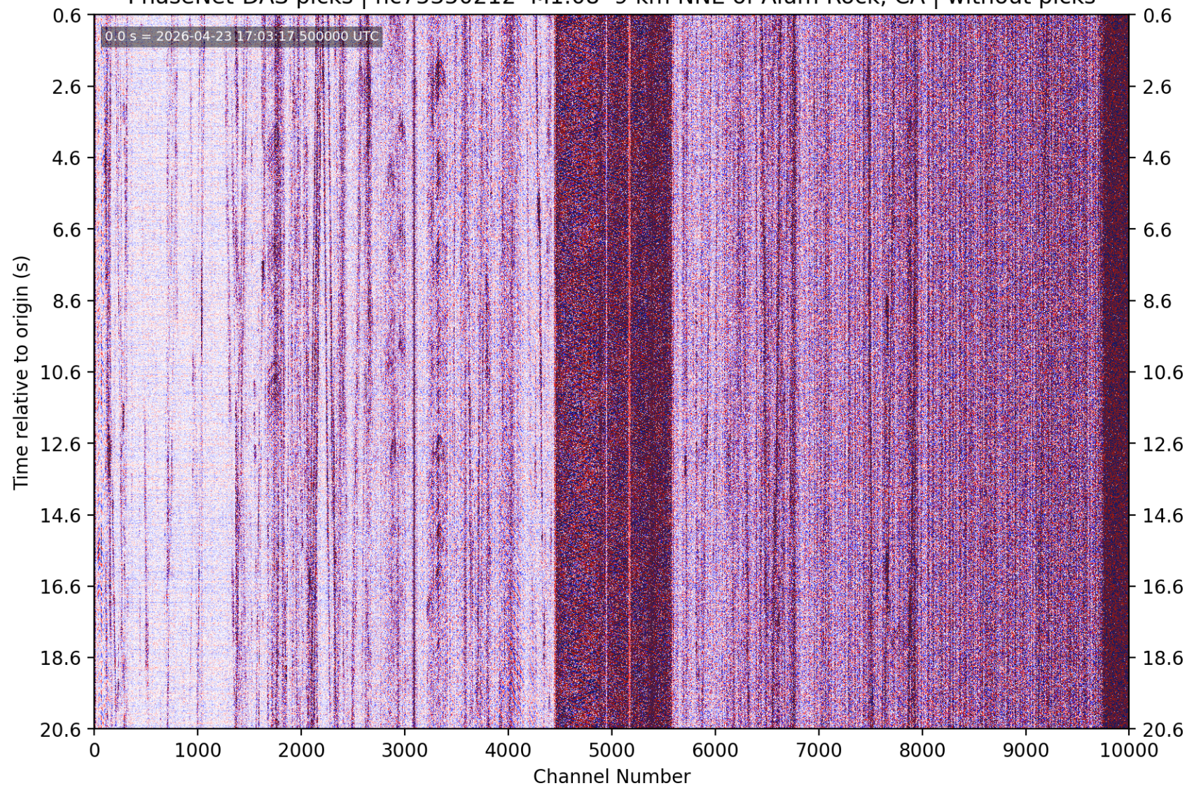
PhaseNet-DAS picks | nc75350212 M1.08 9 km NNE of Alum Rock, CA | without picks
