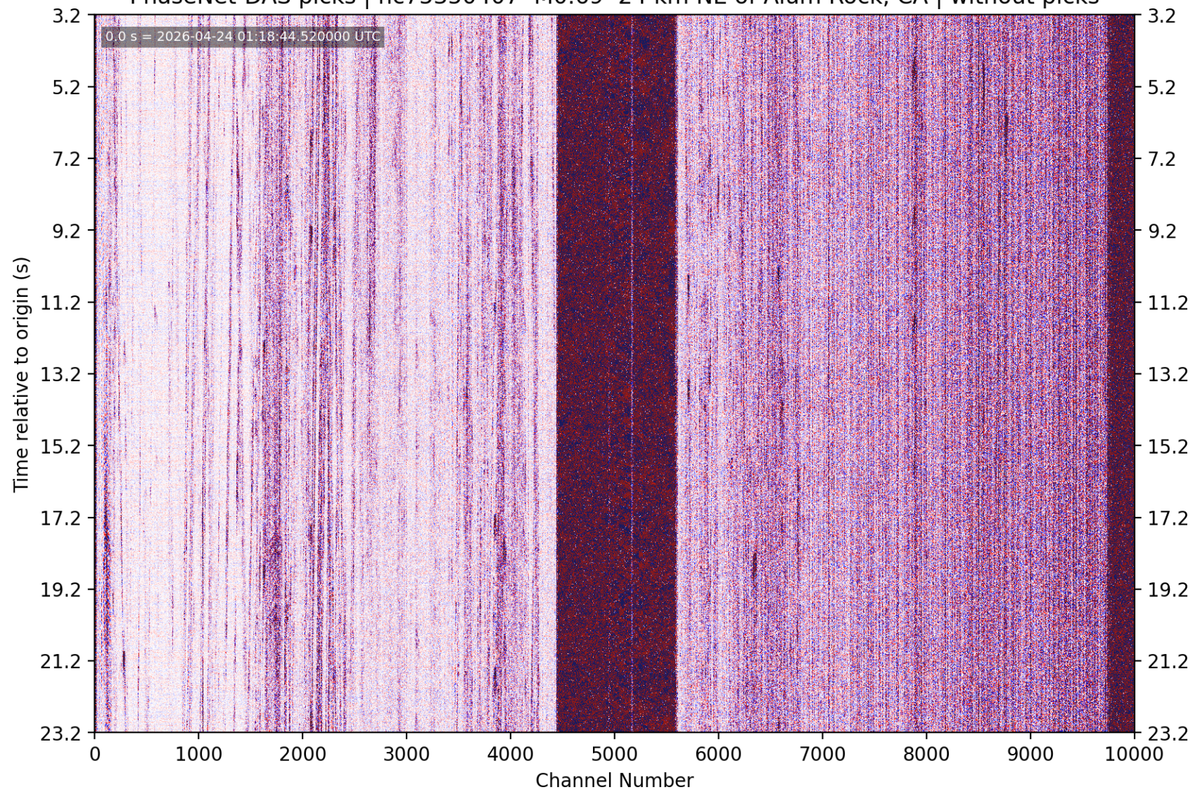
PhaseNet-DAS picks | nc75350407 M0.69 24 km NE of Alum Rock, CA | without picks
