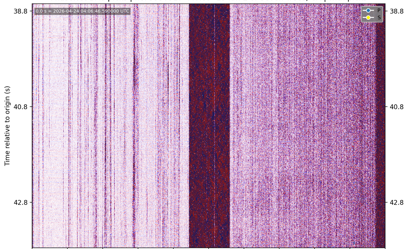
PhaseNet-DAS picks | nc75350517 M0.89 15 km E of Seven Trees, CA | without picks
