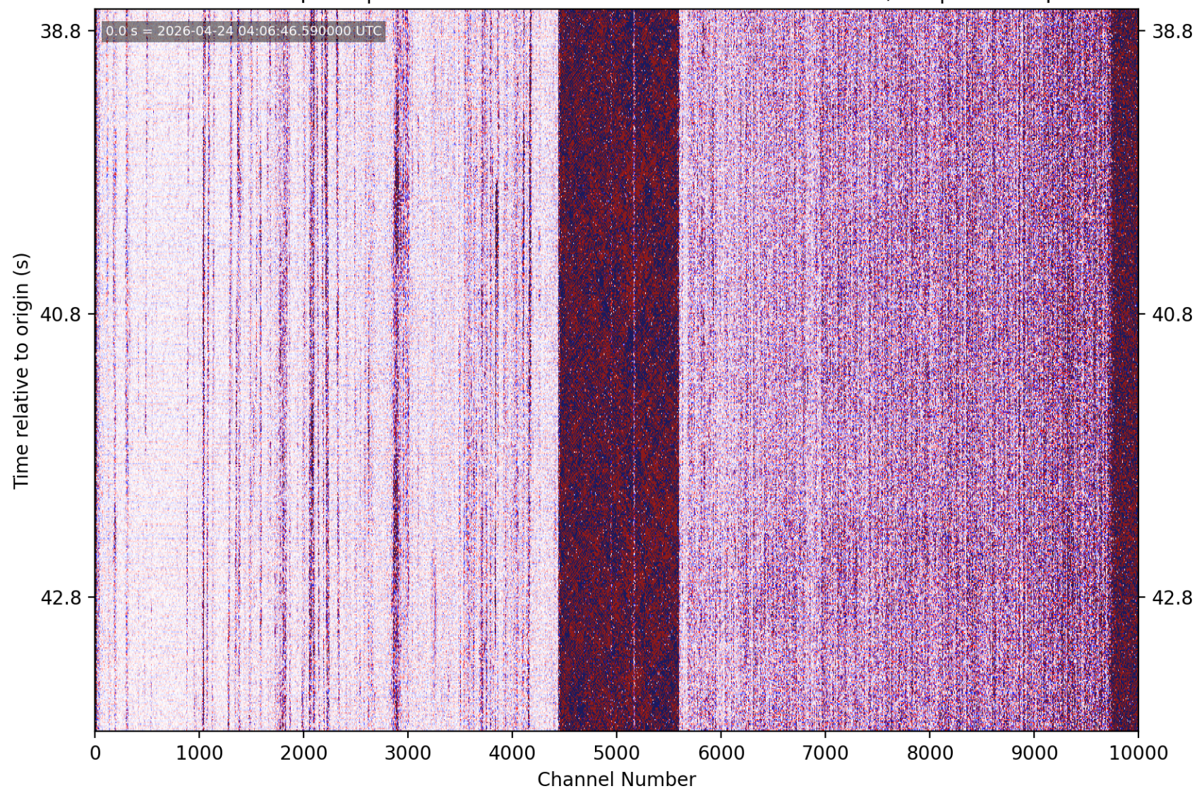
PhaseNet-DAS picks | nc75350517 M0.89 15 km E of Seven Trees, CA | without picks
