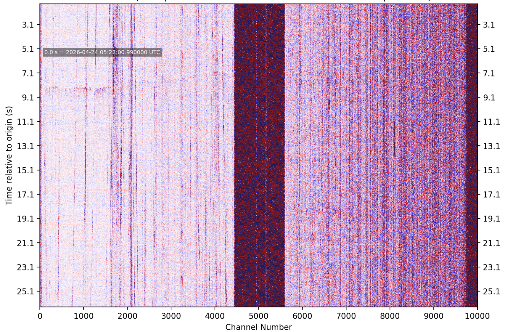
PhaseNet-DAS picks | nc75350542 M0.58 5 km SE of Pacifica, CA | without picks
