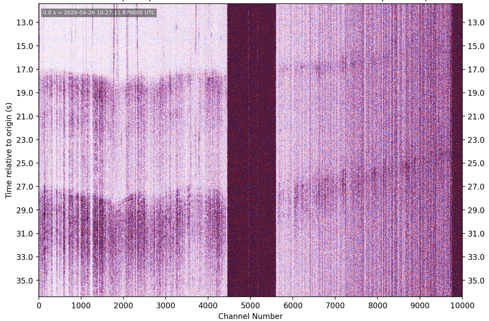
PhaseNet-DAS picks | nc75351867 M2.62 16 km E of Seven Trees, CA | without picks
