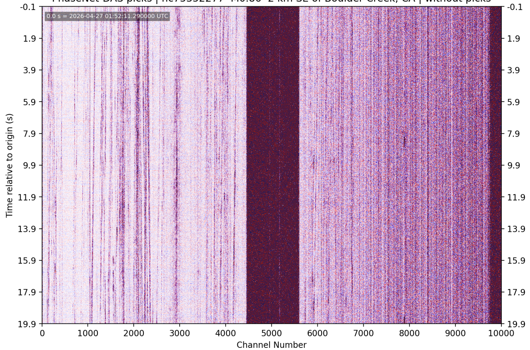
PhaseNet-DAS picks | nc75352277 M0.86 2 km SE of Boulder Creek, CA | without picks
