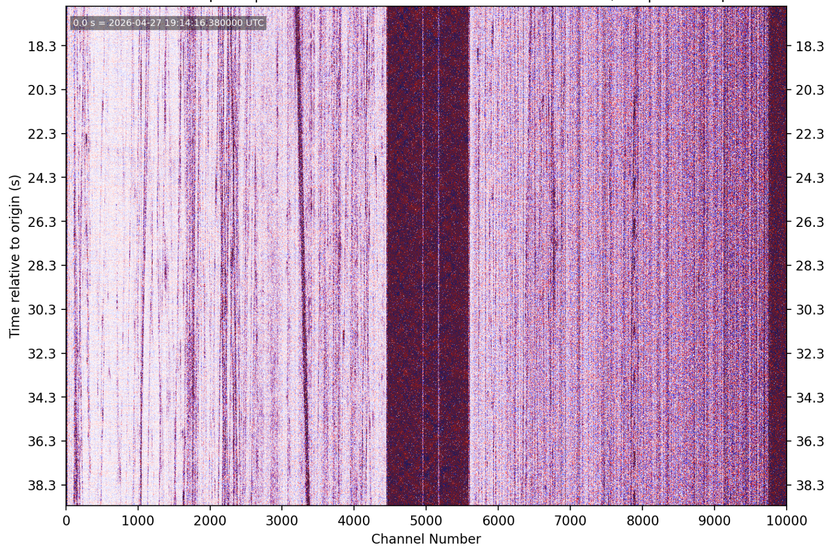
PhaseNet-DAS picks | nc75352722 M1.45 2 km SE of Santa Clara, CA | without picks
