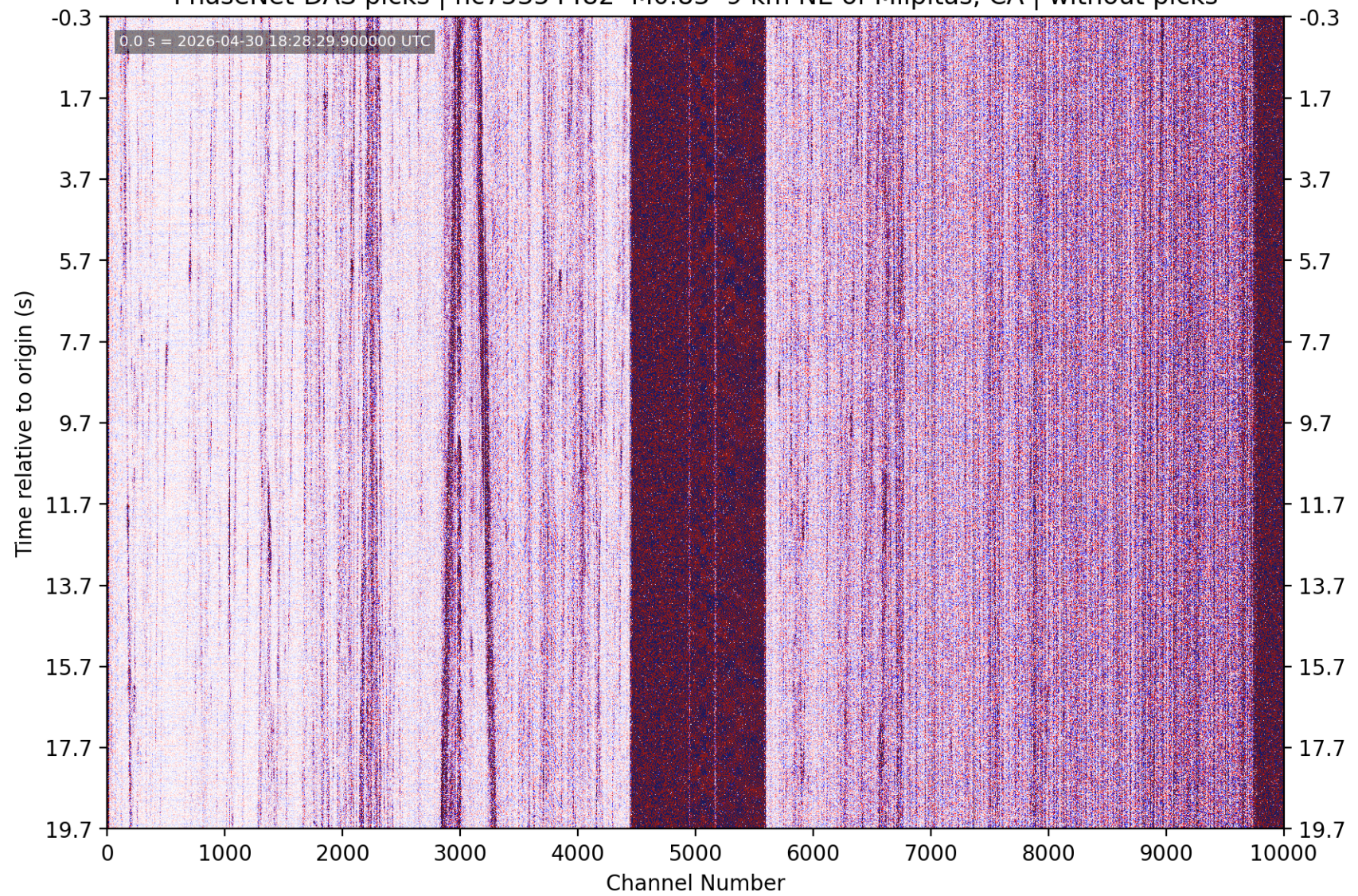
PhaseNet-DAS picks | nc75354482 M0.83 9 km NE of Milpitas, CA | without picks
